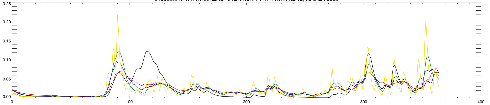
01030500 MATTAWAMKEAG RIVER NEAR MATTAWAMKEAG, MAINE : 2004
