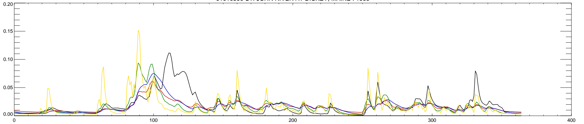
01010500 ST. JOHN RIVER AT DICKEY, MAINE : 2000
