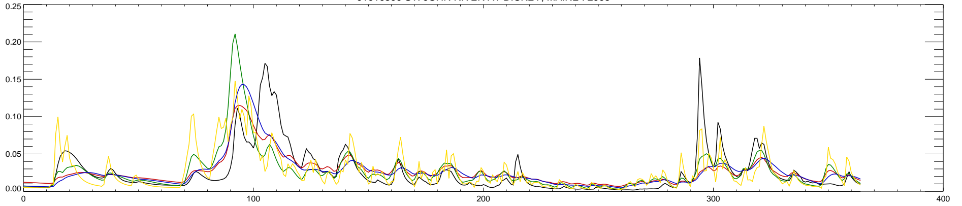
01010500 ST. JOHN RIVER AT DICKEY, MAINE : 2007
