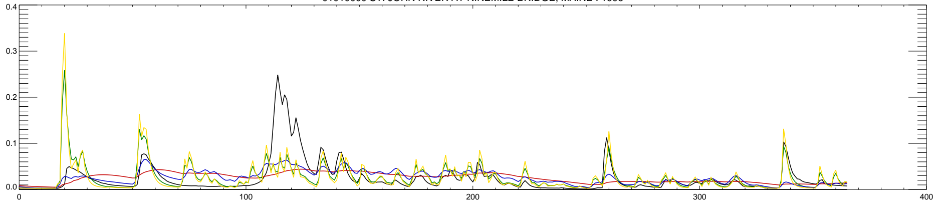
01010000 ST. JOHN RIVER AT NINEMILE BRIDGE, MAINE : 1997
