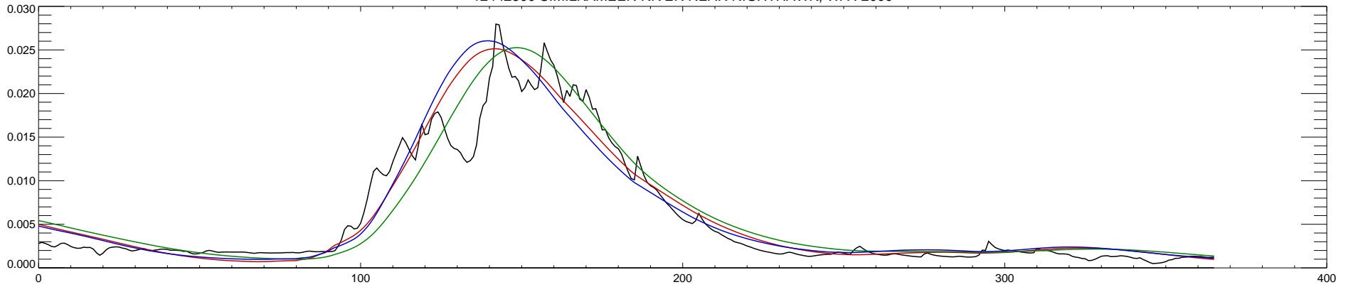
12442500 SIMILKAMEEN RIVER NEAR NIGHTHAWK, WA : 2001
