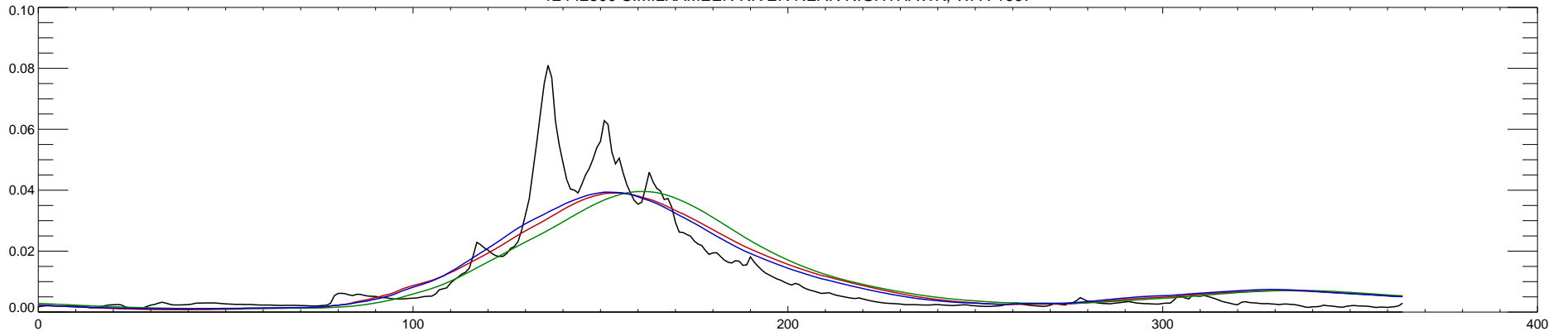
12442500 SIMILKAMEEN RIVER NEAR NIGHTHAWK, WA : 1998
