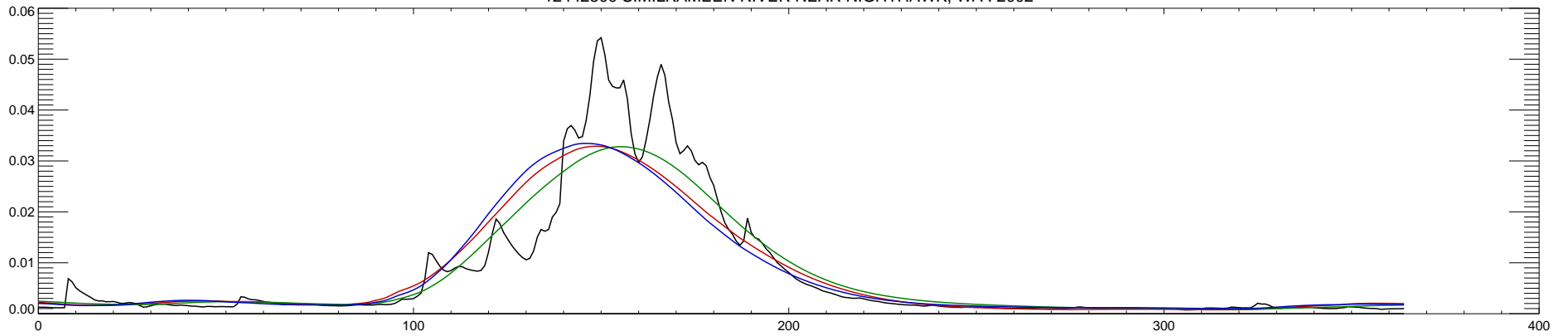
12442500 SIMILKAMEEN RIVER NEAR NIGHTHAWK, WA : 2003
