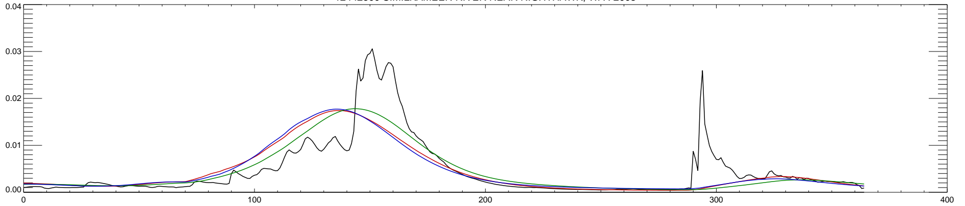
12442500 SIMILKAMEEN RIVER NEAR NIGHTHAWK, WA : 2004
