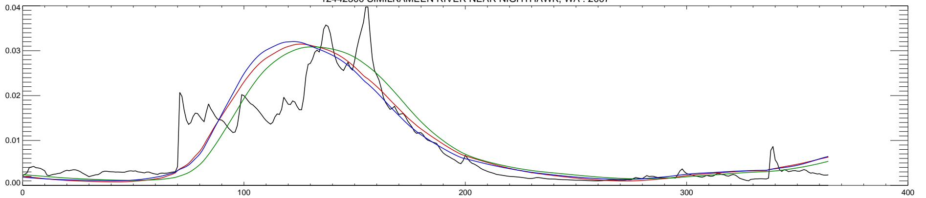
12442500 SIMILKAMEEN RIVER NEAR NIGHTHAWK, WA : 2007
