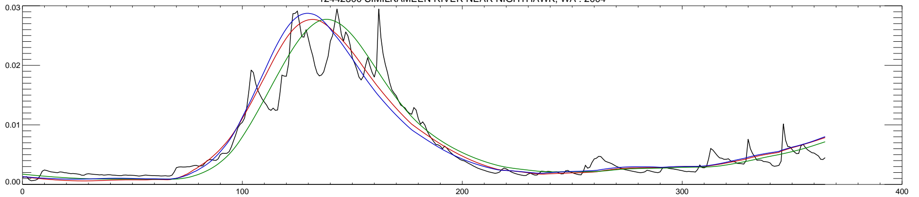
12442500 SIMILKAMEEN RIVER NEAR NIGHTHAWK, WA : 2004
