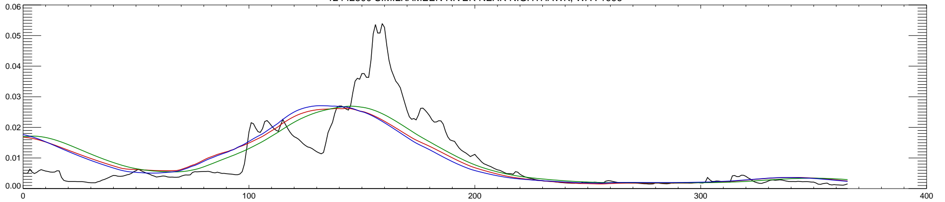
12442500 SIMILKAMEEN RIVER NEAR NIGHTHAWK, WA : 1997
