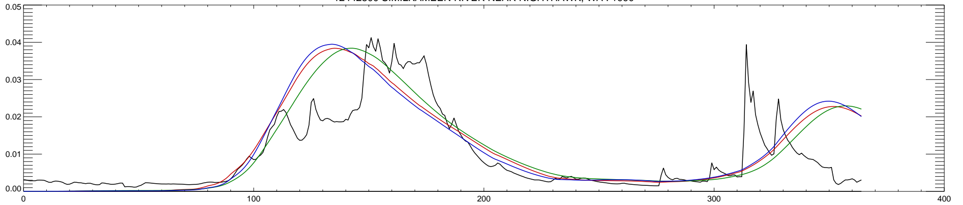
12442500 SIMILKAMEEN RIVER NEAR NIGHTHAWK, WA : 1991
