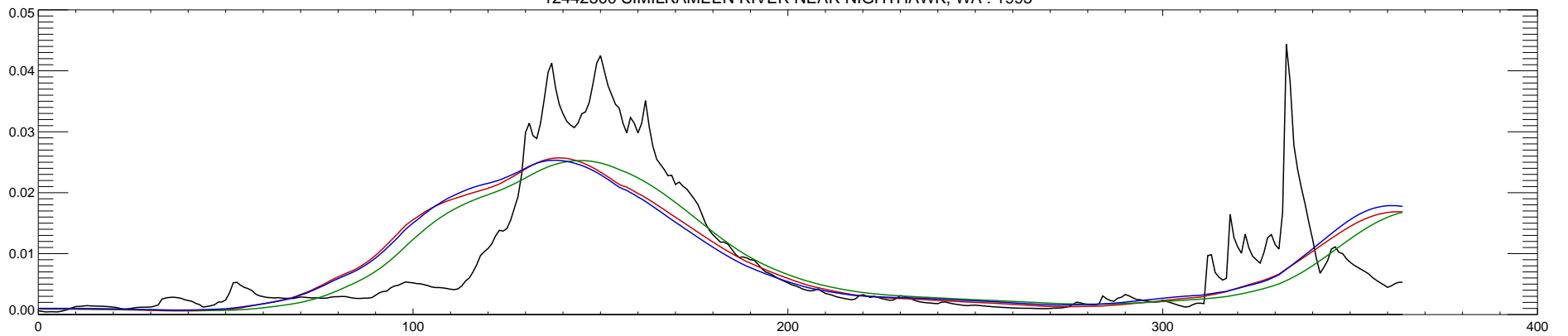
12442500 SIMILKAMEEN RIVER NEAR NIGHTHAWK, WA : 1995
