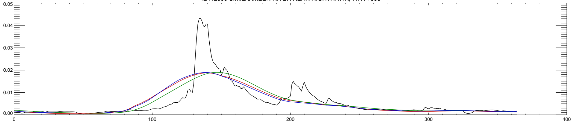
12442500 SIMILKAMEEN RIVER NEAR NIGHTHAWK, WA : 1994
