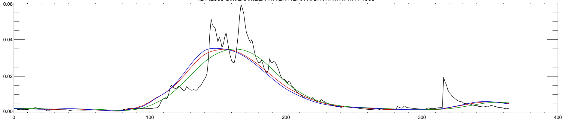
12442500 SIMILKAMEEN RIVER NEAR NIGHTHAWK, WA : 2000
