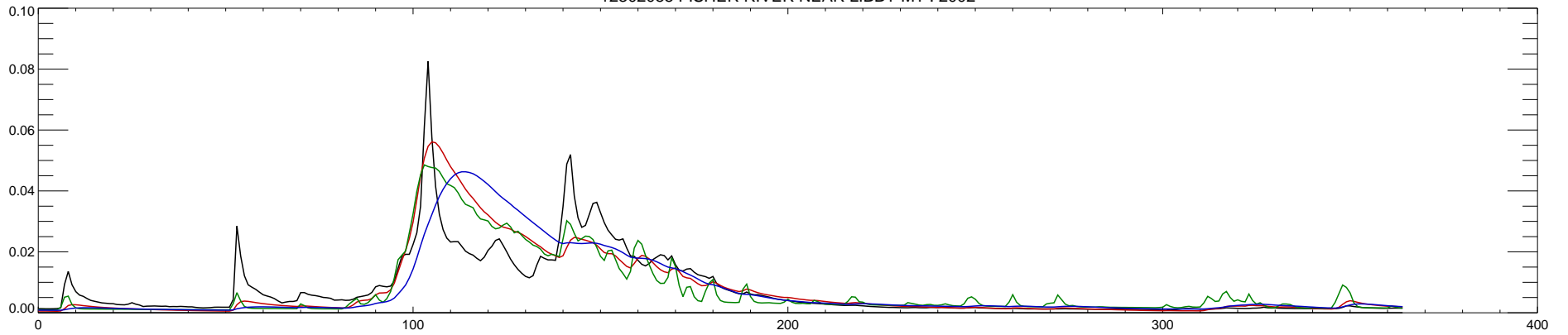
12302055 FISHER RIVER NEAR LIBBY MT : 2003
