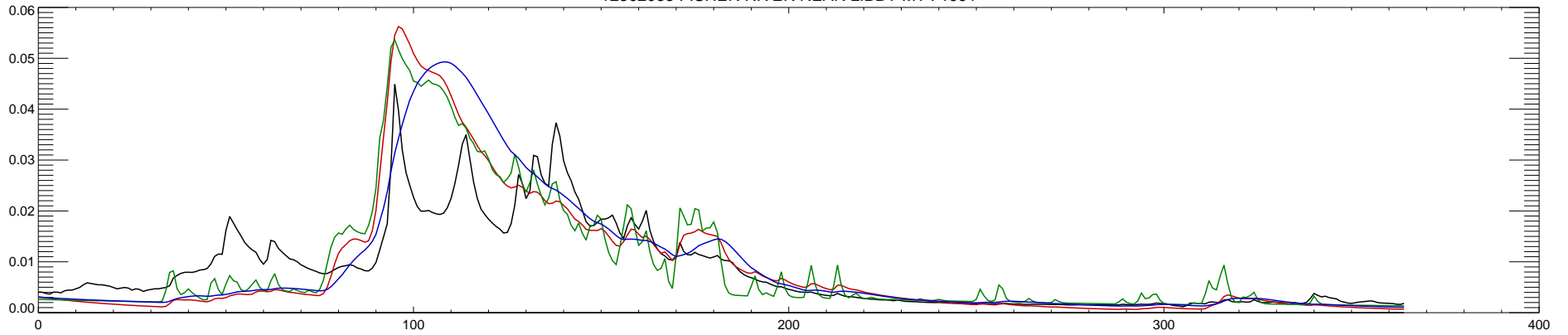
12302055 FISHER RIVER NEAR LIBBY MT : 1992
