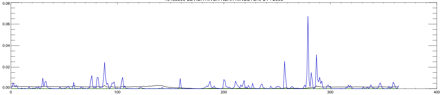
10183500 SEVIER RIVER NEAR KINGSTON, UT : 2007
