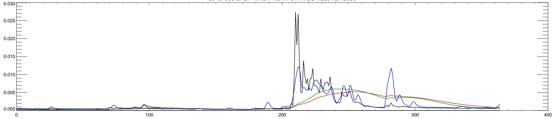
09497500 SALT RIVER NEAR CHRYSOTILE, AZ : 2007
