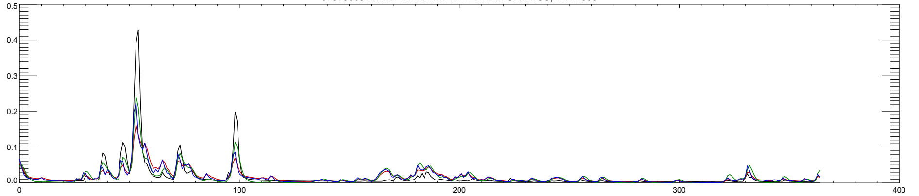
07378500 AMITE RIVER NEAR DENHAM SPRINGS, LA : 2004
