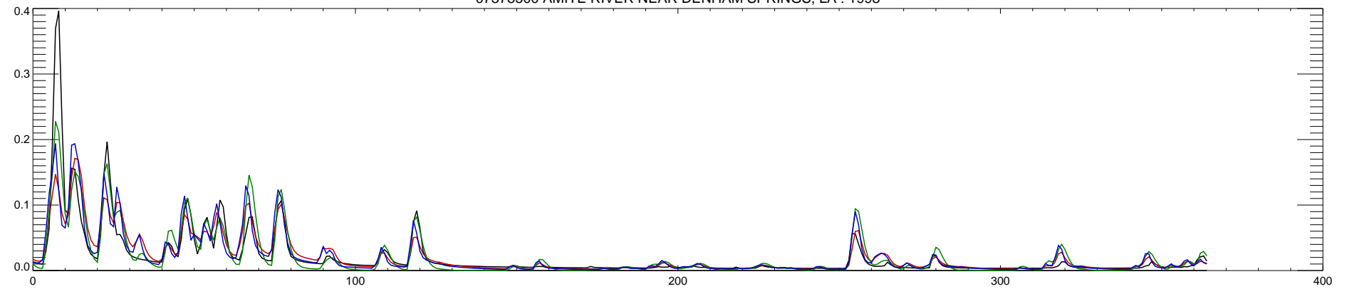
07378500 AMITE RIVER NEAR DENHAM SPRINGS, LA : 1998
