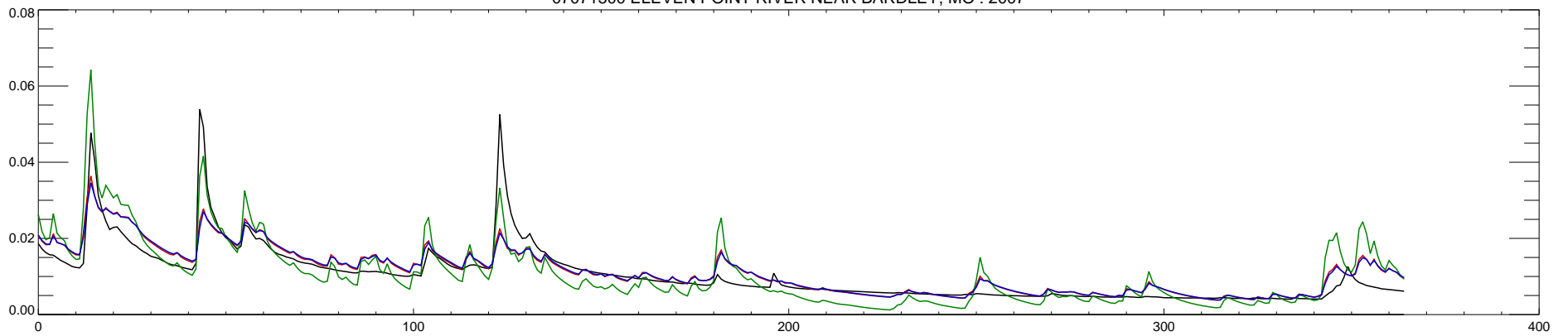
07071500 ELEVEN POINT RIVER NEAR BARDLEY, MO : 2007
