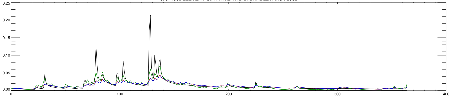
07071500 ELEVEN POINT RIVER NEAR BARDLEY, MO : 2003
