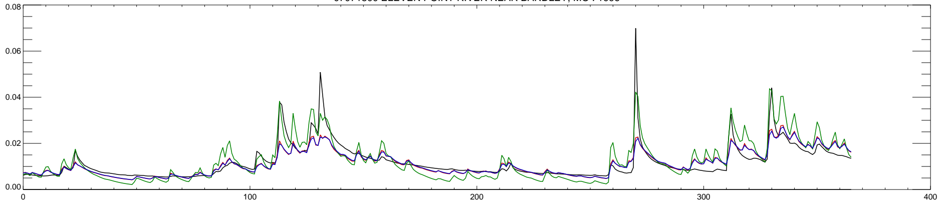
07071500 ELEVEN POINT RIVER NEAR BARDLEY, MO : 1997
