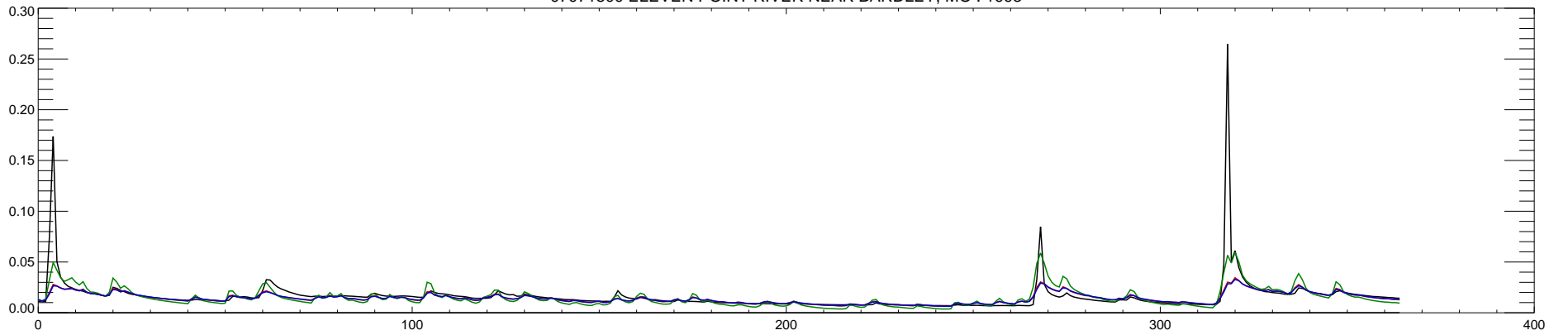
07071500 ELEVEN POINT RIVER NEAR BARDLEY, MO : 1994
