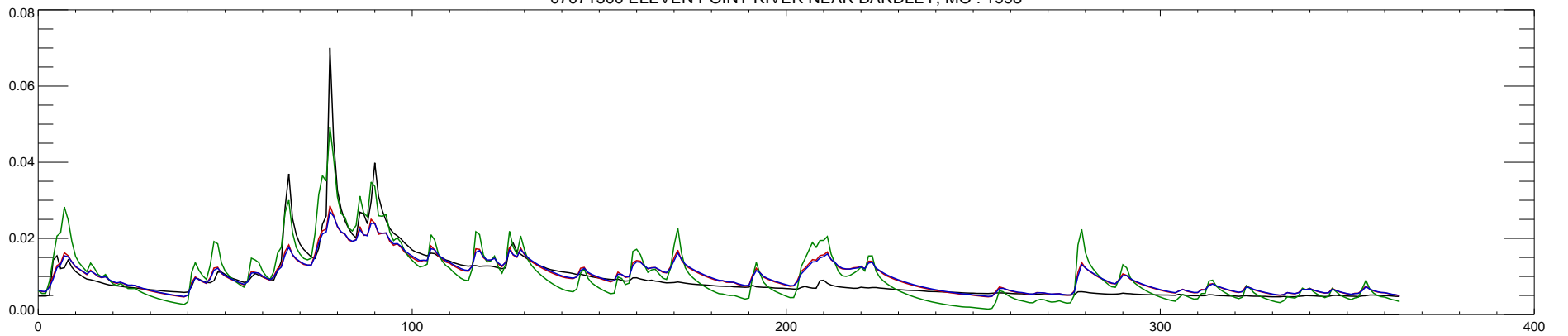
07071500 ELEVEN POINT RIVER NEAR BARDLEY, MO : 1998
