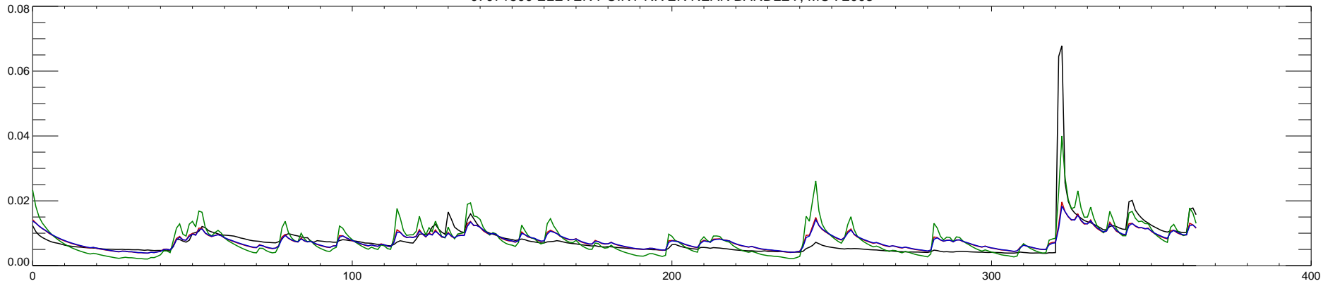
07071500 ELEVEN POINT RIVER NEAR BARDLEY, MO : 2004
