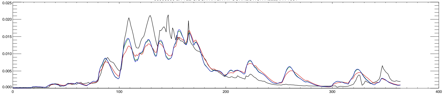
06606600 LITTLE SIOUX RIVER AT CORRECTIONVILLE, IA : 1992
