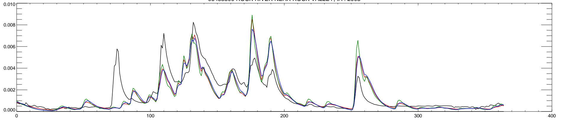
06483500 ROCK RIVER NEAR ROCK VALLEY, IA : 2004
