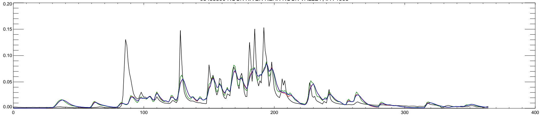
06483500 ROCK RIVER NEAR ROCK VALLEY, IA : 1994
