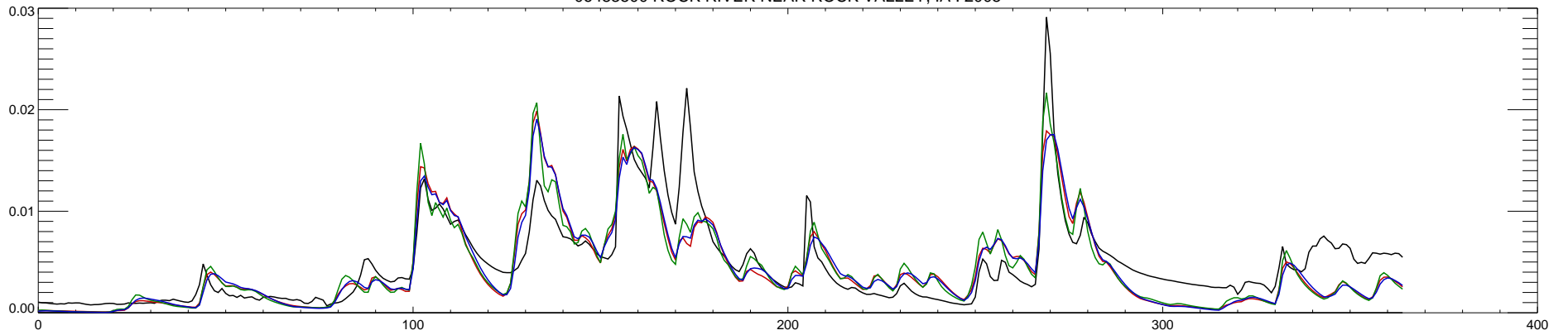
06483500 ROCK RIVER NEAR ROCK VALLEY, IA : 2006
