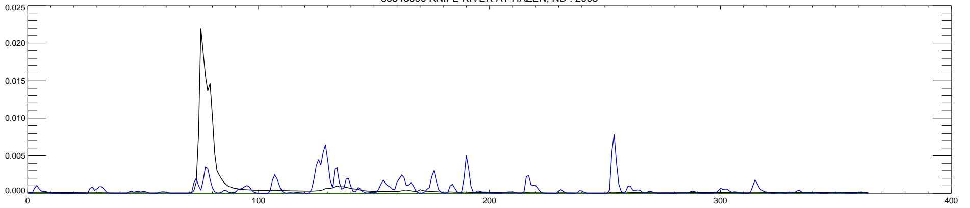
06340500 KNIFE RIVER AT HAZEN, ND : 2004
