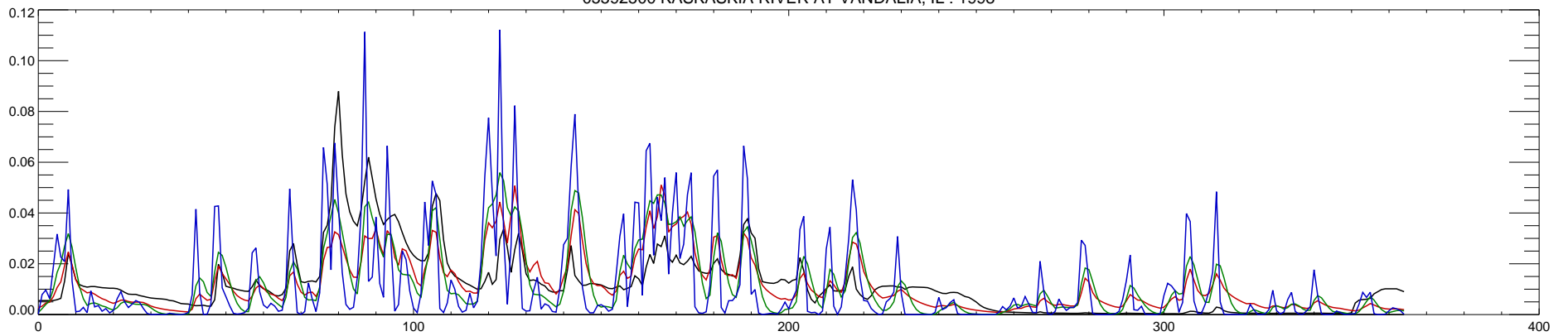
05592500 KASKASKIA RIVER AT VANDALIA, IL : 1998
