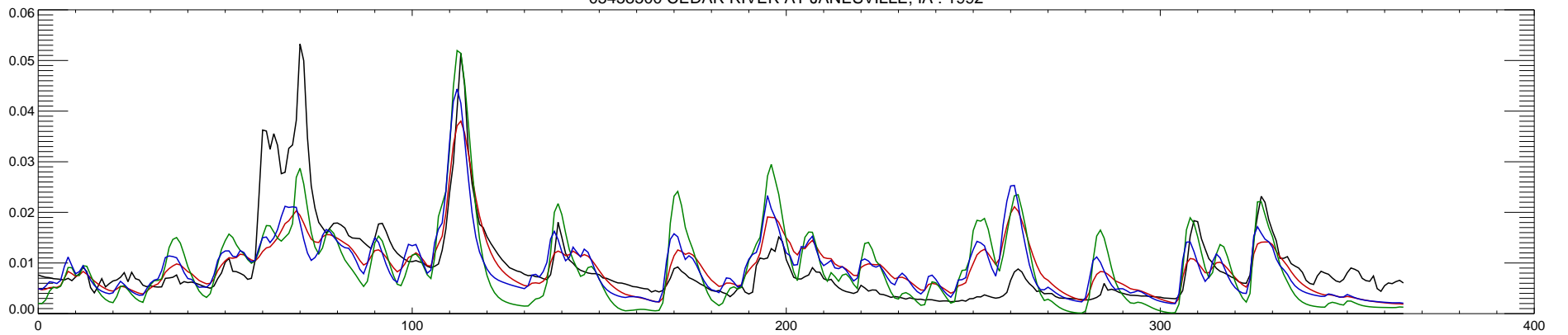
05458500 CEDAR RIVER AT JANESVILLE, IA : 1992
