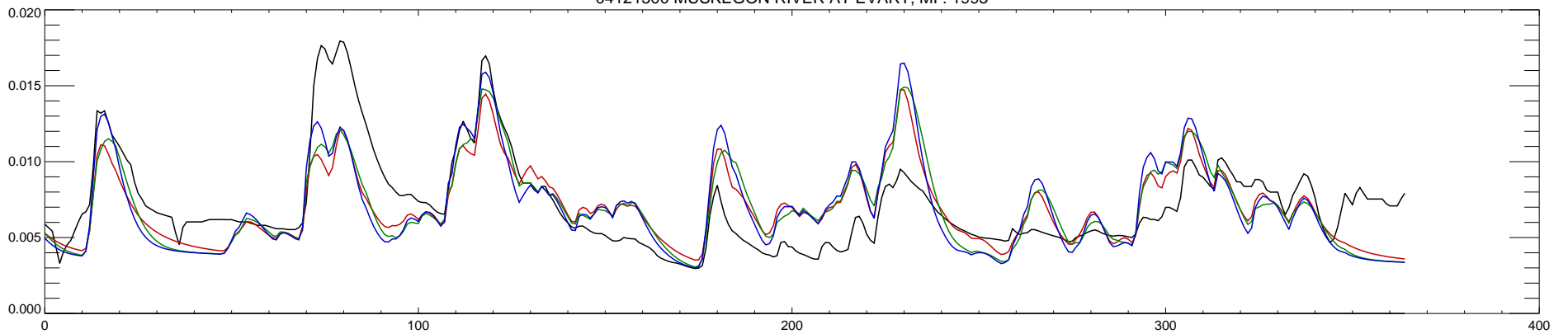
04121500 MUSKEGON RIVER AT EVART, MI : 1995
