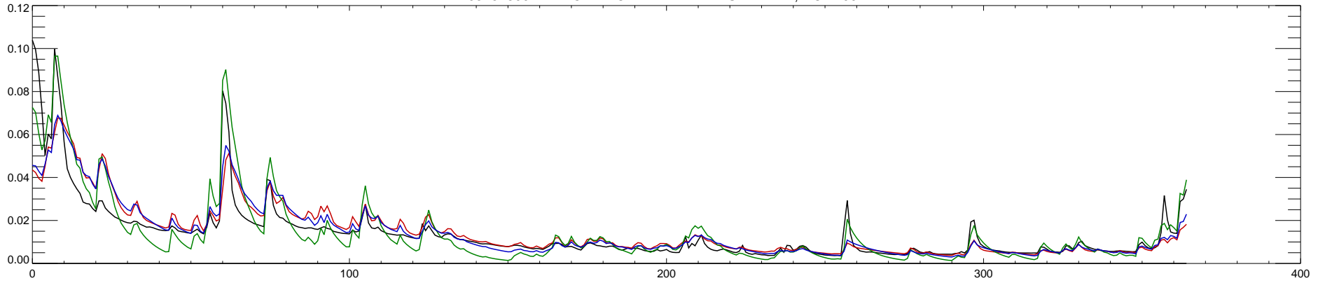
03451500 FRENCH BROAD RIVER AT ASHEVILLE, NC : 2007
