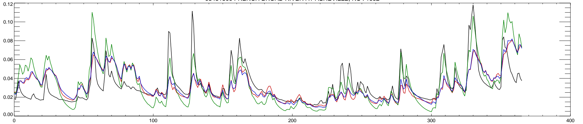
03451500 FRENCH BROAD RIVER AT ASHEVILLE, NC : 1992
