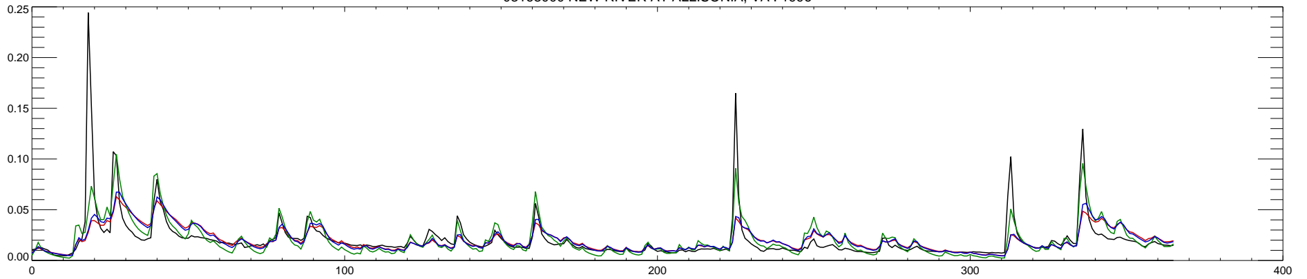
03168000 NEW RIVER AT ALLISONIA, VA : 1997
