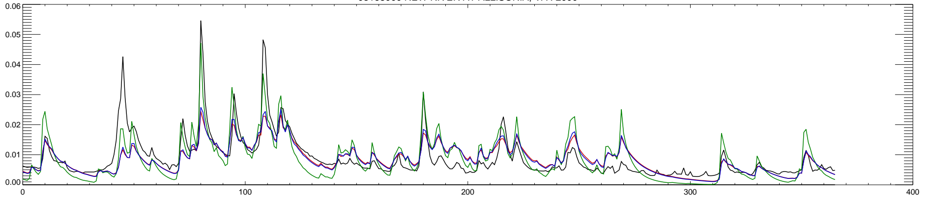
03168000 NEW RIVER AT ALLISONIA, VA : 2001
