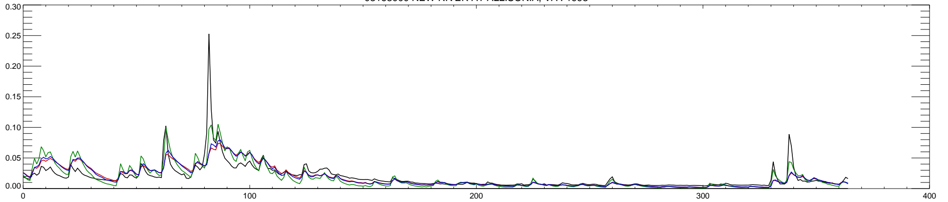
03168000 NEW RIVER AT ALLISONIA, VA : 1994
