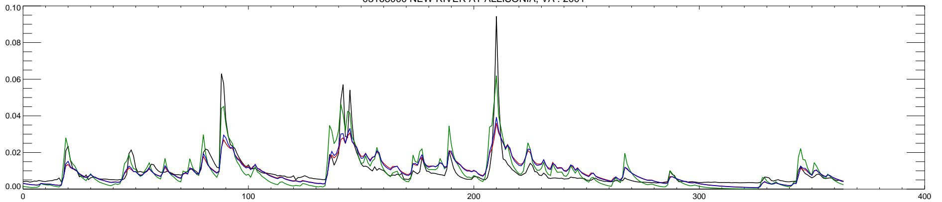
03168000 NEW RIVER AT ALLISONIA, VA : 2001
