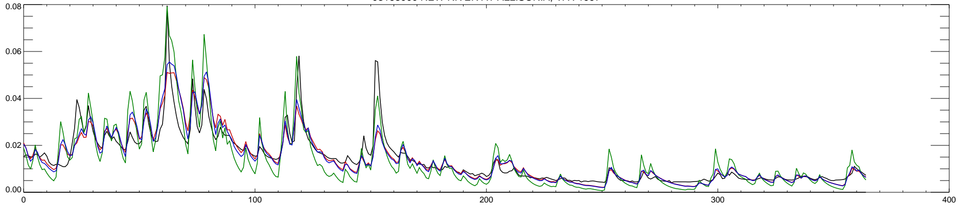
03168000 NEW RIVER AT ALLISONIA, VA : 1998
