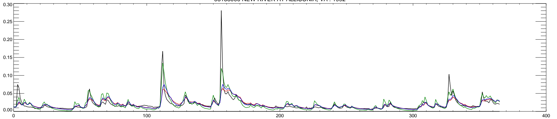
03168000 NEW RIVER AT ALLISONIA, VA : 1992
