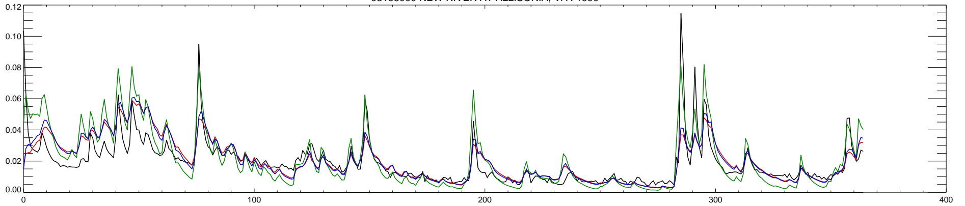
03168000 NEW RIVER AT ALLISONIA, VA : 1991
