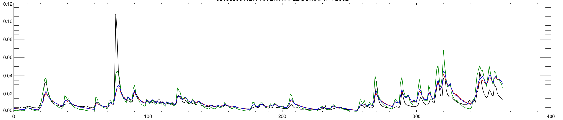
03168000 NEW RIVER AT ALLISONIA, VA : 2003
