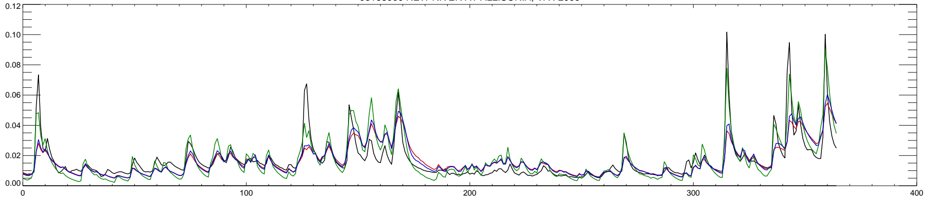
03168000 NEW RIVER AT ALLISONIA, VA : 2009
