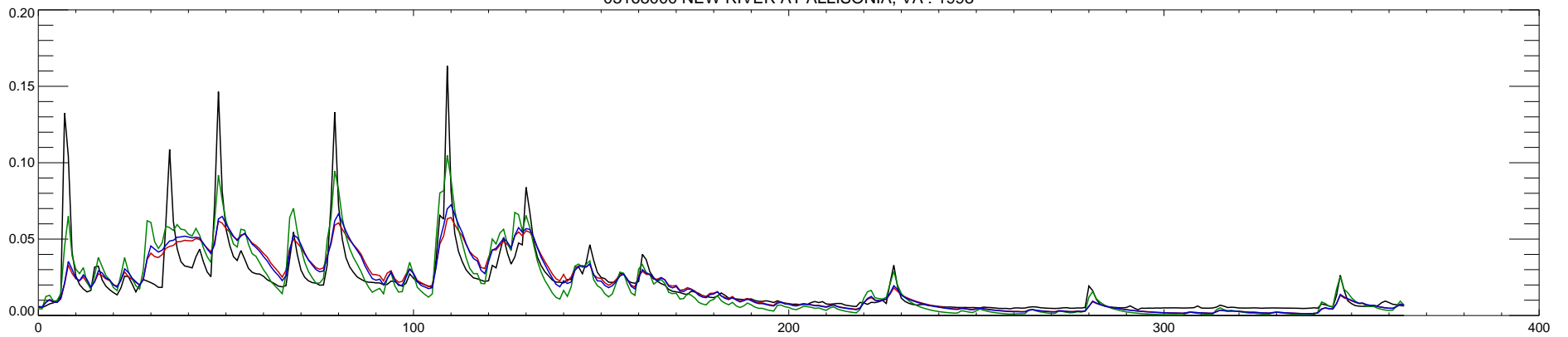
03168000 NEW RIVER AT ALLISONIA, VA : 1998
