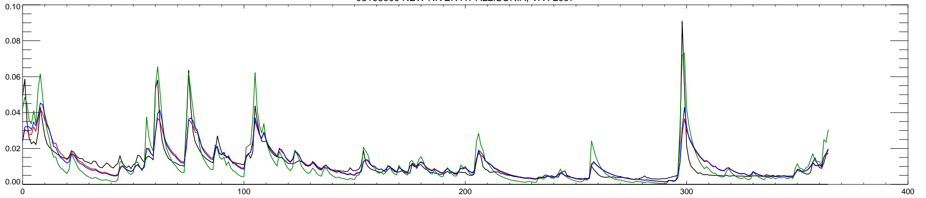
03168000 NEW RIVER AT ALLISONIA, VA : 2007
