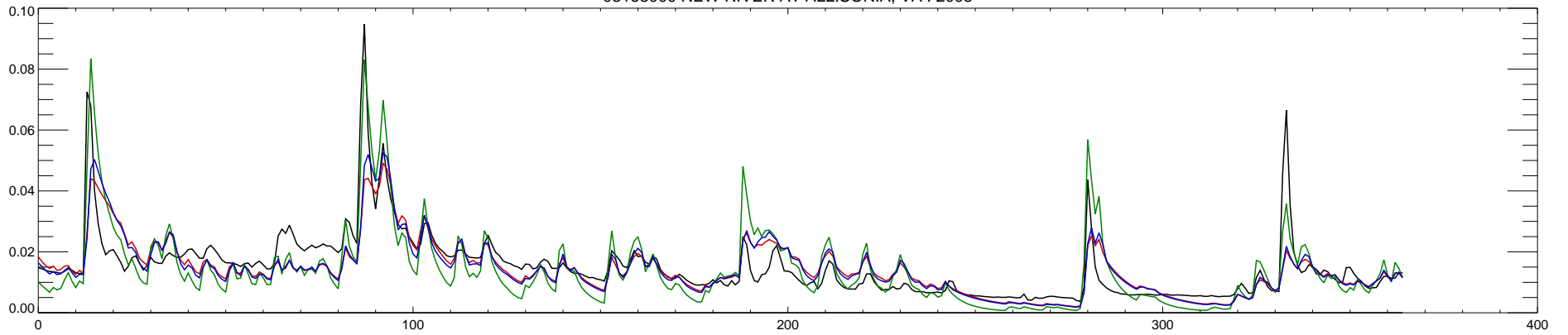
03168000 NEW RIVER AT ALLISONIA, VA : 2006
