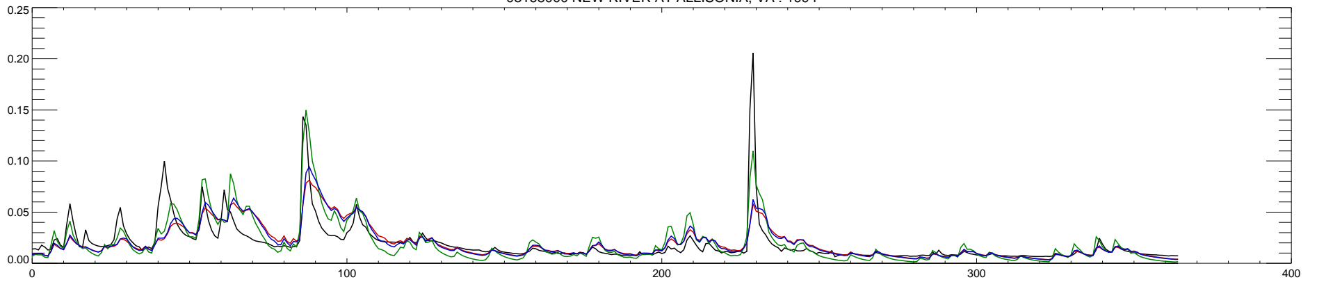
03168000 NEW RIVER AT ALLISONIA, VA : 1995
