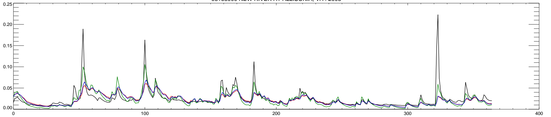
03168000 NEW RIVER AT ALLISONIA, VA : 2004
