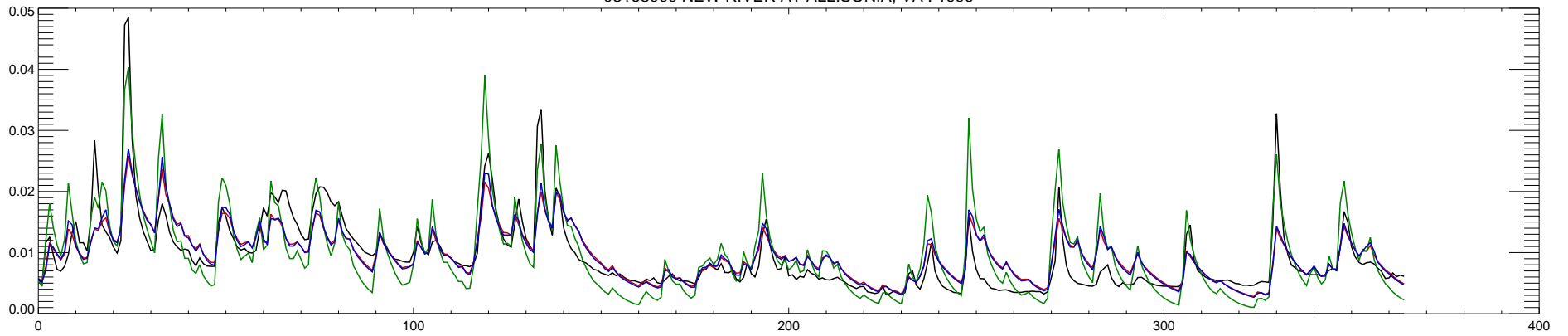
03168000 NEW RIVER AT ALLISONIA, VA : 2000
