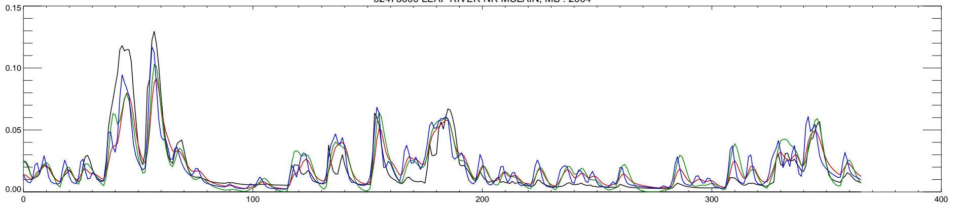
02475000 LEAF RIVER NR MCLAIN, MS : 2004
