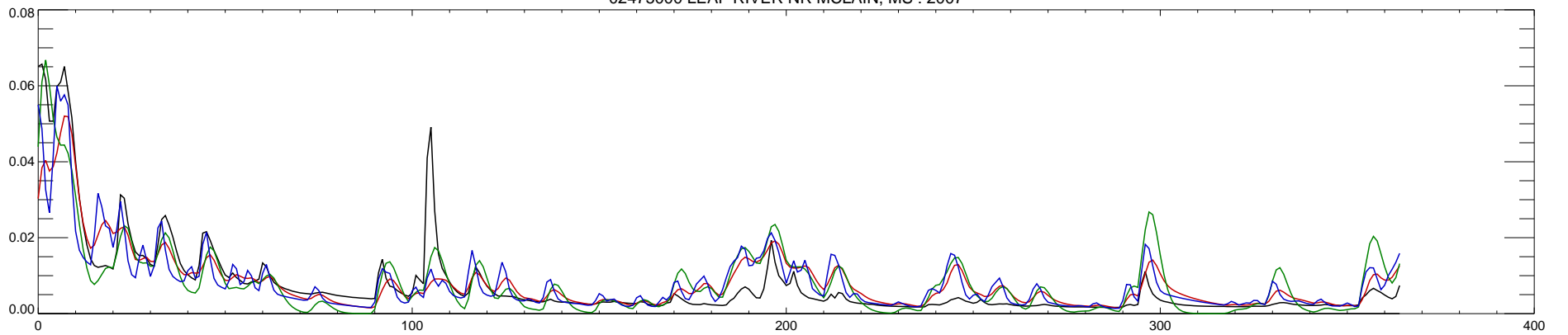
02475000 LEAF RIVER NR MCLAIN, MS : 2007
