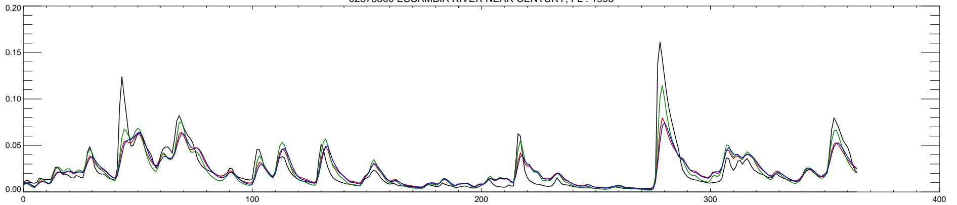
02375500 ESCAMBIA RIVER NEAR CENTURY, FL : 1995
