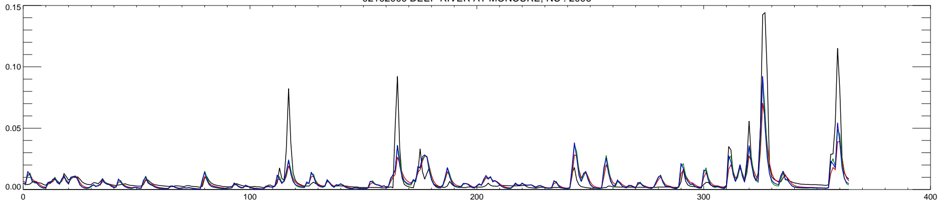
02102000 DEEP RIVER AT MONCURE, NC : 2007
