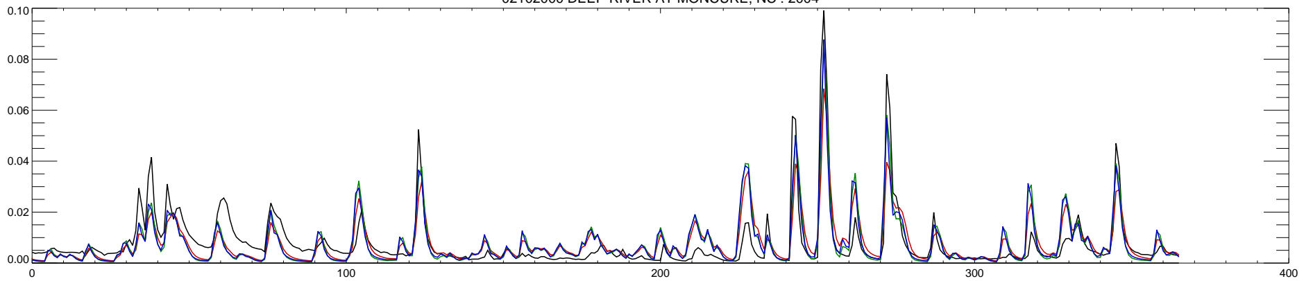
02102000 DEEP RIVER AT MONCURE, NC : 2004
