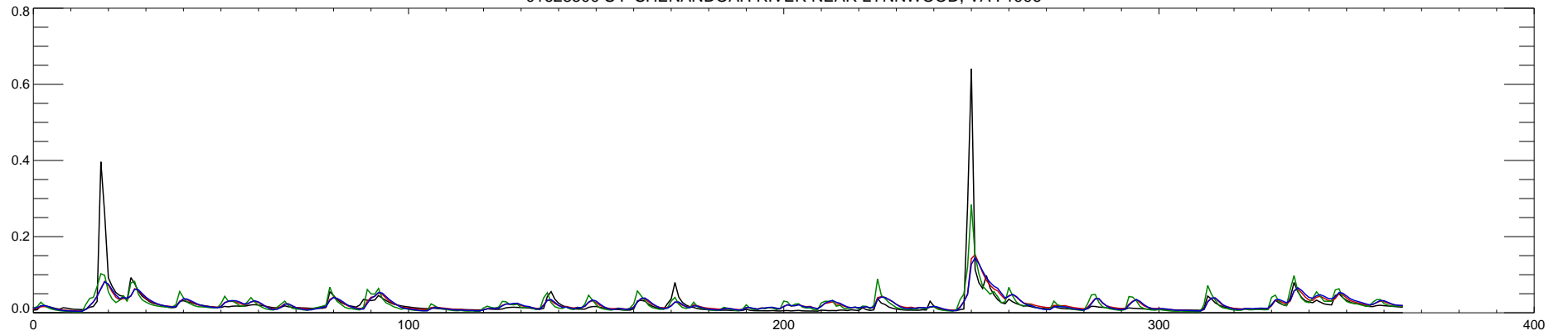
01628500 S F SHENANDOAH RIVER NEAR LYNNWOOD, VA : 1997
