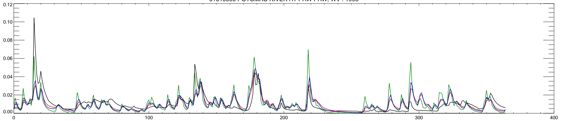
01610000 POTOMAC RIVER AT PAW PAW, WV : 1995
