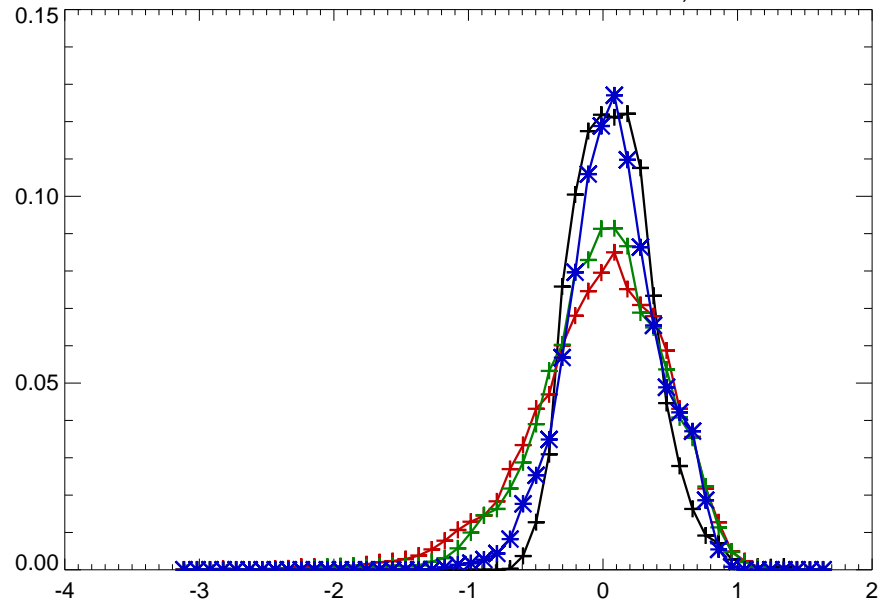
03164000 NEW RIVER NEAR GALAX, VA
