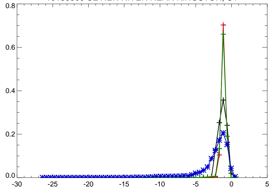
10183500 SEVIER RIVER NEAR KINGSTON, UT
