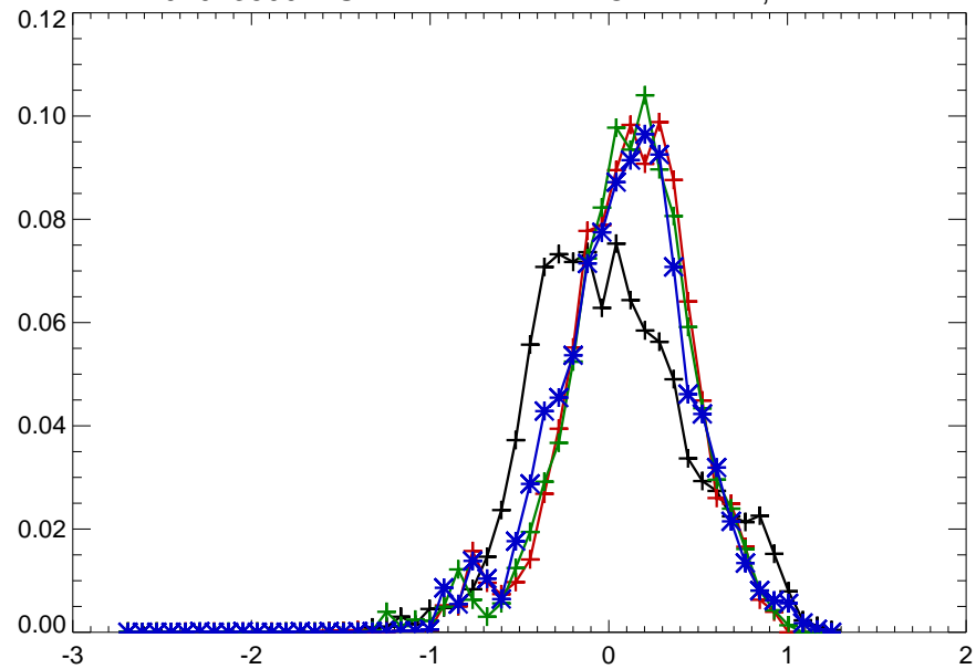
01013500 FISH RIVER NEAR FORT KENT, MAINE
