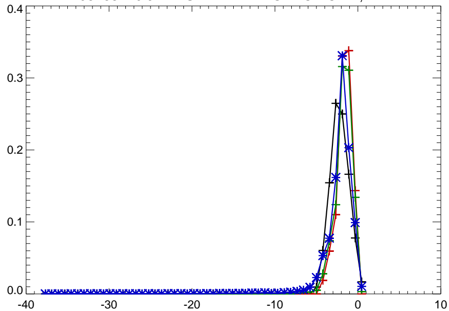
06468170 JAMES RIVER NR GRACE CITY, ND
