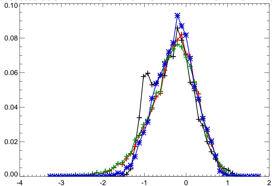
01608500 SOUTH BRANCH POTOMAC RIVER NEAR SPRINGFIELD, WV
