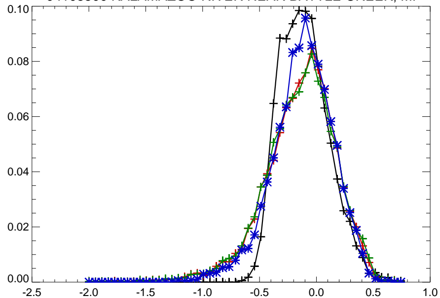
04105500 KALAMAZOO RIVER NEAR BATTLE CREEK, MI
