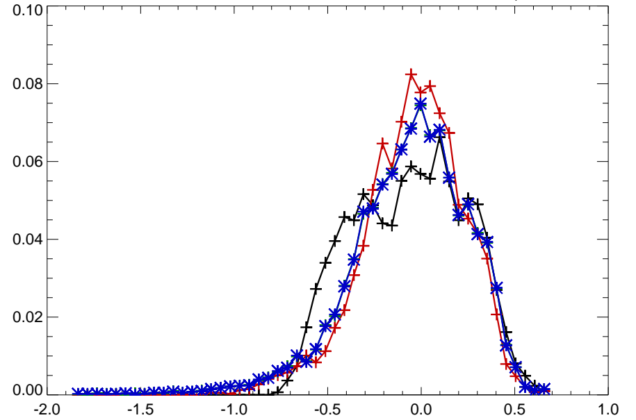
05520500 KANKAKEE RIVER AT MOMENCE, IL
