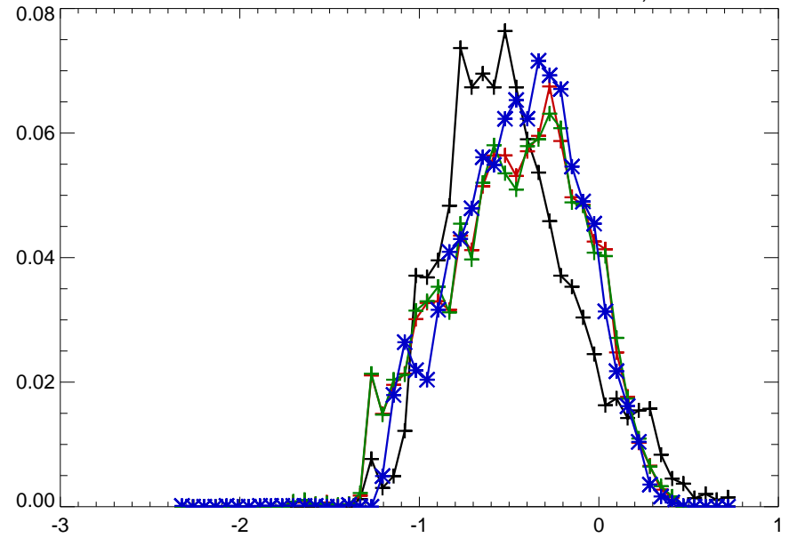
05286000 RUM RIVER NEAR ST. FRANCIS, MN
