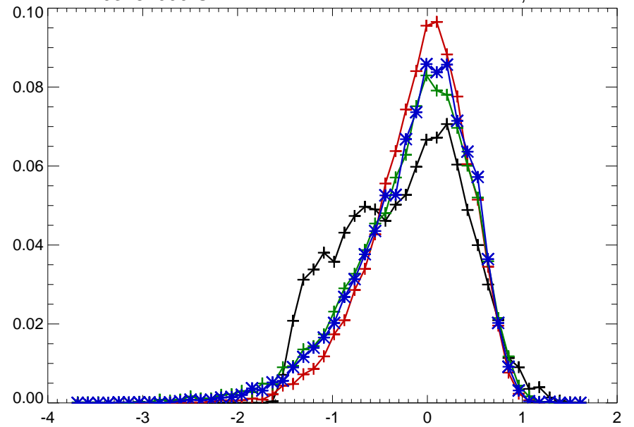
03184000 GREENBRIER RIVER AT HILLDALE, WV
