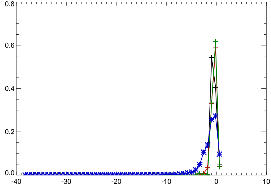
06225500 WIND RIVER NEAR CROWHEART, WY
