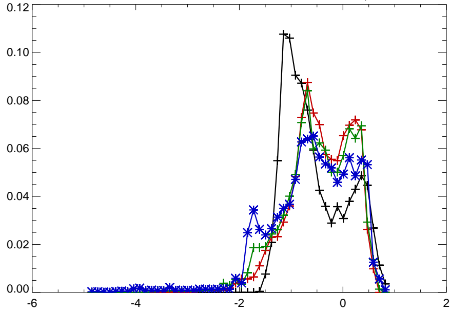
12404500 KETTLE RIVER NEAR LAURIER, WA
