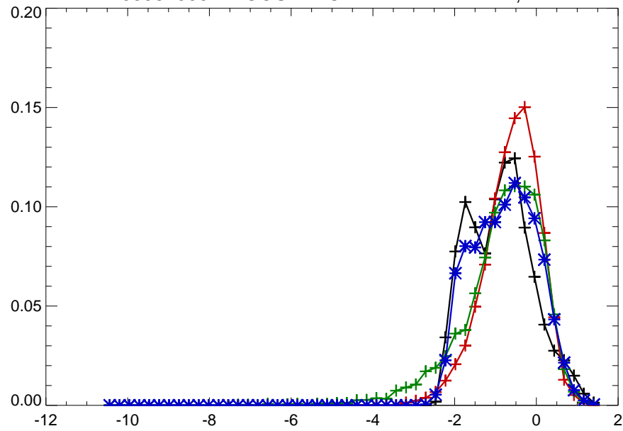
05587000 MACOUPIN CREEK NEAR KANE, IL
