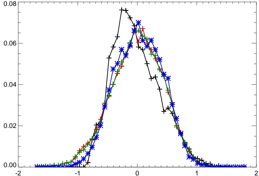
01421000 EAST BRANCH DELAWARE RIVER AT FISHS EDDY NY
