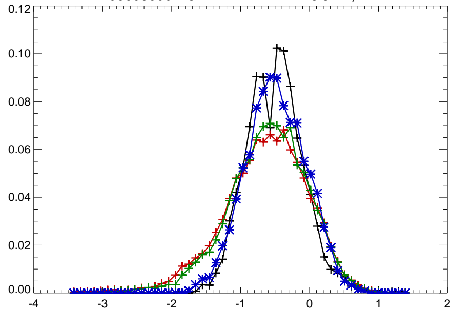
06609500 BOYER RIVER AT LOGAN, IA
