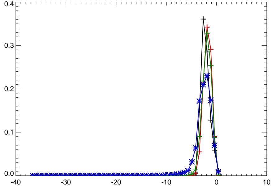
06334500 LITTLE MISSOURI R AT CAMP CROOK, SD
