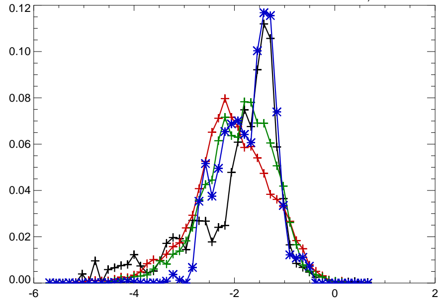
06873000 SF SOLOMON R AB WEBSTER RE, KS
