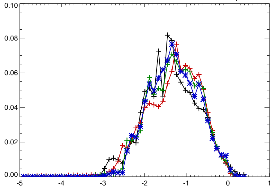
06480000 BIG SIOUX RIVER NEAR BROOKINGS, SD
