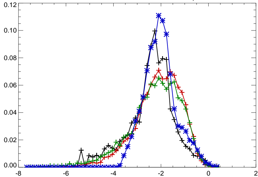
07141200 PAWNEE R AT ROZEL, KS
