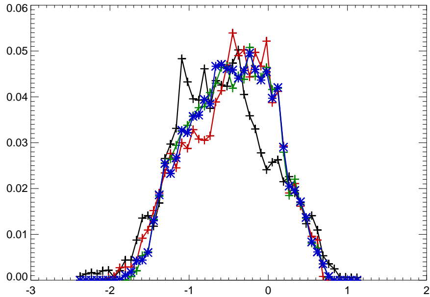
02296750 PEACE RIVER AT ARCADIA FL
