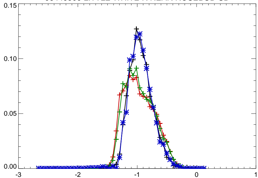
06449500 LITTLE WHITE R NEAR ROSEBUD SD
