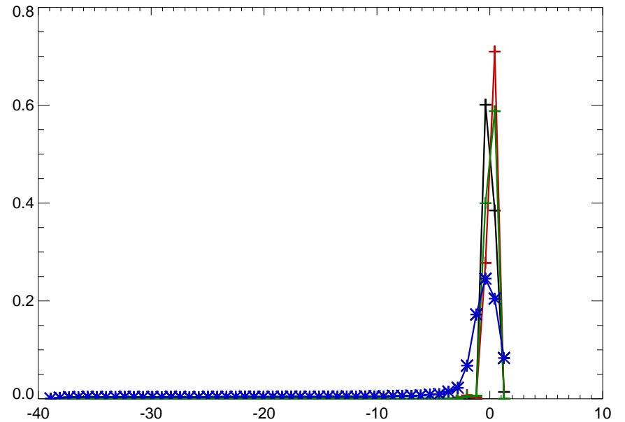
13011000 SNAKE RIVER NR MORAN WY
