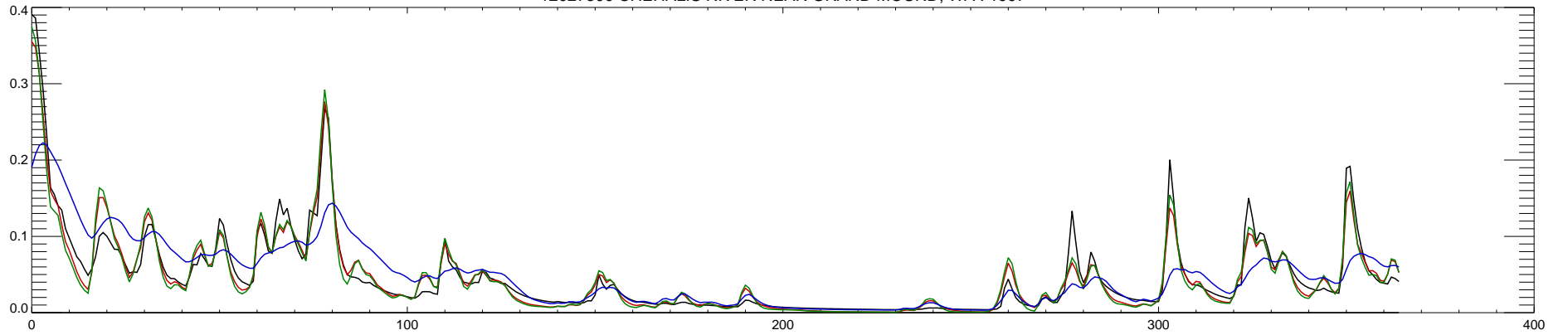
12027500 CHEHALIS RIVER NEAR GRAND MOUND, WA : 1998
