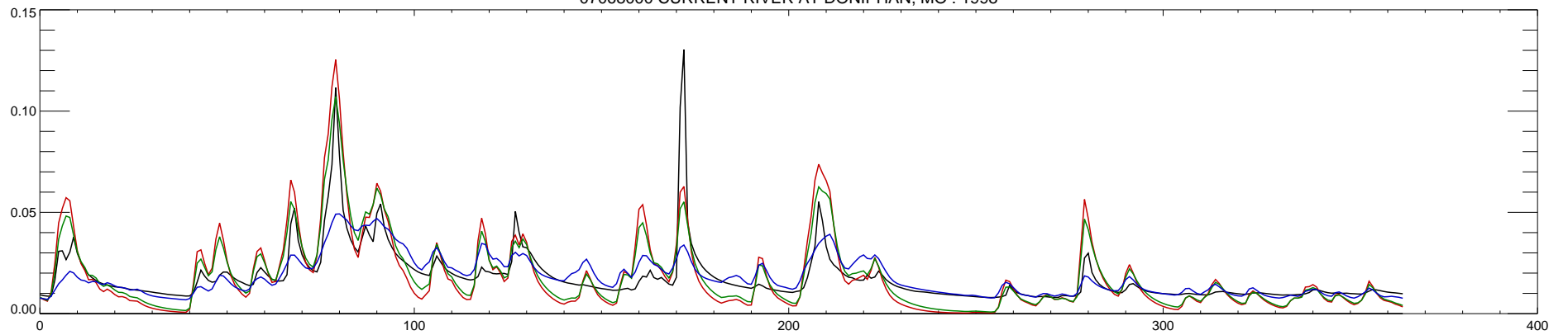
07068000 CURRENT RIVER AT DONIPHAN, MO : 1998
