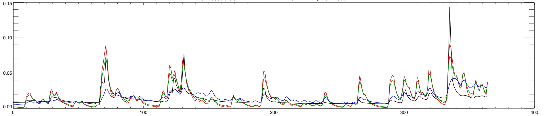
07068000 CURRENT RIVER AT DONIPHAN, MO : 2007
