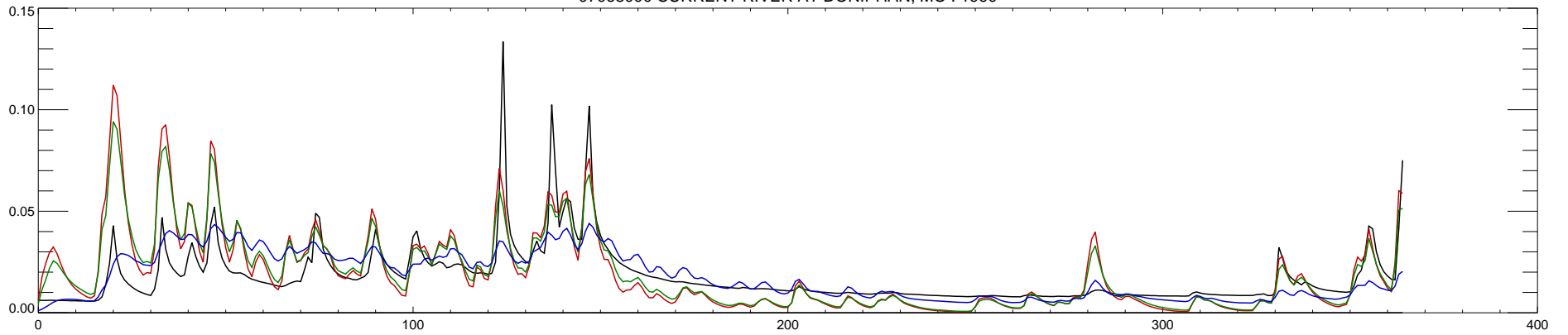
07068000 CURRENT RIVER AT DONIPHAN, MO : 1991
