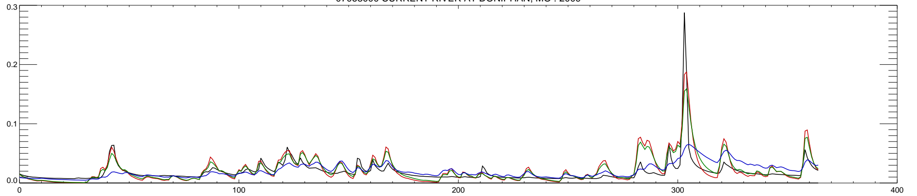
07068000 CURRENT RIVER AT DONIPHAN, MO : 2009
