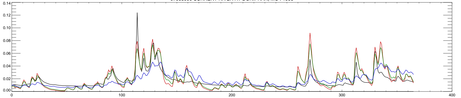
07068000 CURRENT RIVER AT DONIPHAN, MO : 1997
