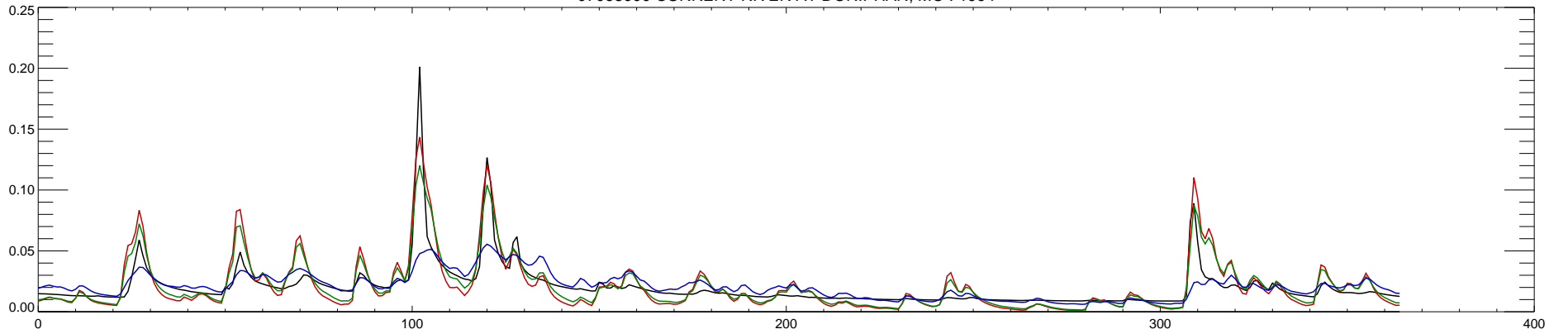
07068000 CURRENT RIVER AT DONIPHAN, MO : 1995
