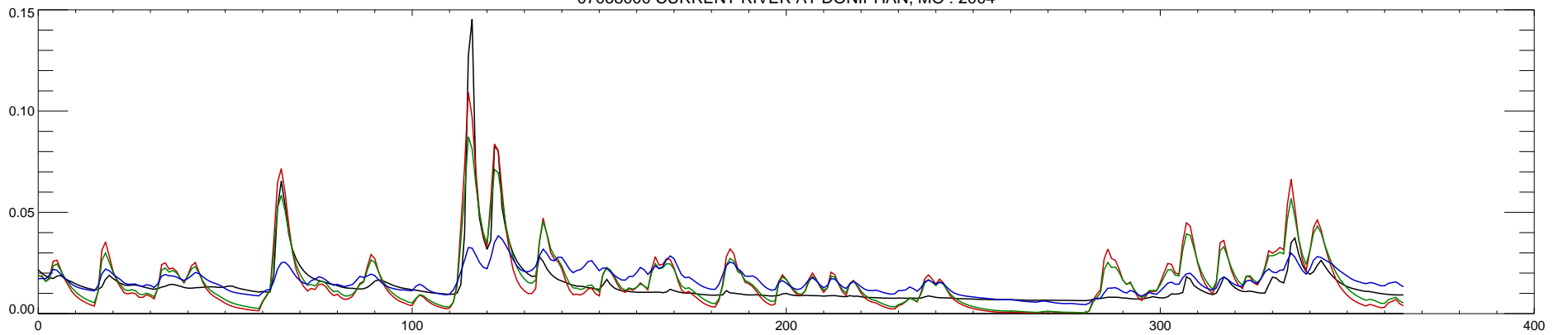
07068000 CURRENT RIVER AT DONIPHAN, MO : 2004
