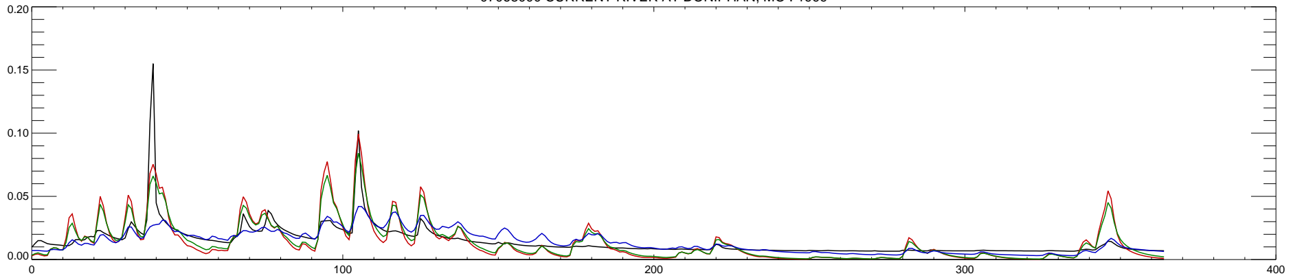
07068000 CURRENT RIVER AT DONIPHAN, MO : 2000
