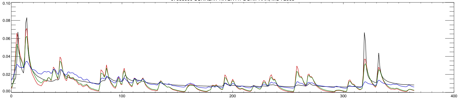
07068000 CURRENT RIVER AT DONIPHAN, MO : 2006
