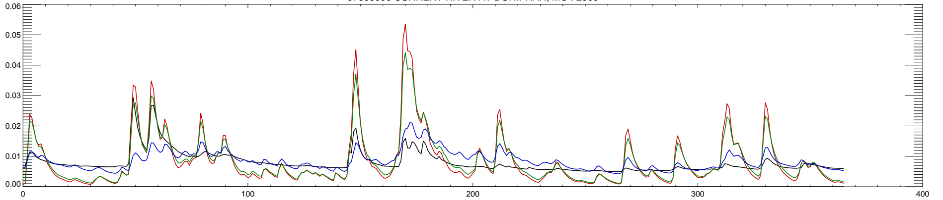
07068000 CURRENT RIVER AT DONIPHAN, MO : 2001
