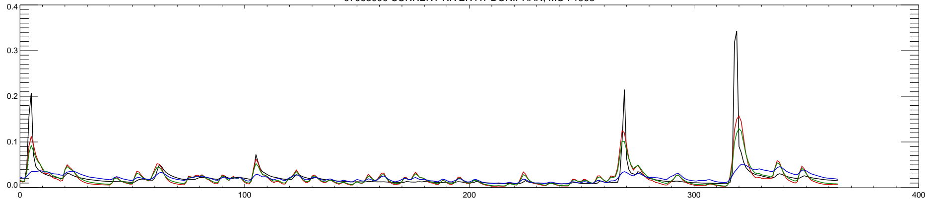
07068000 CURRENT RIVER AT DONIPHAN, MO : 1994
