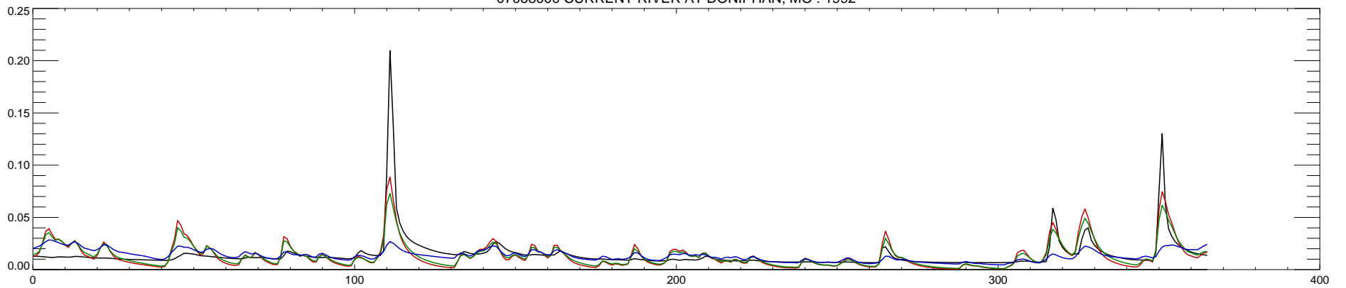
07068000 CURRENT RIVER AT DONIPHAN, MO : 1992
