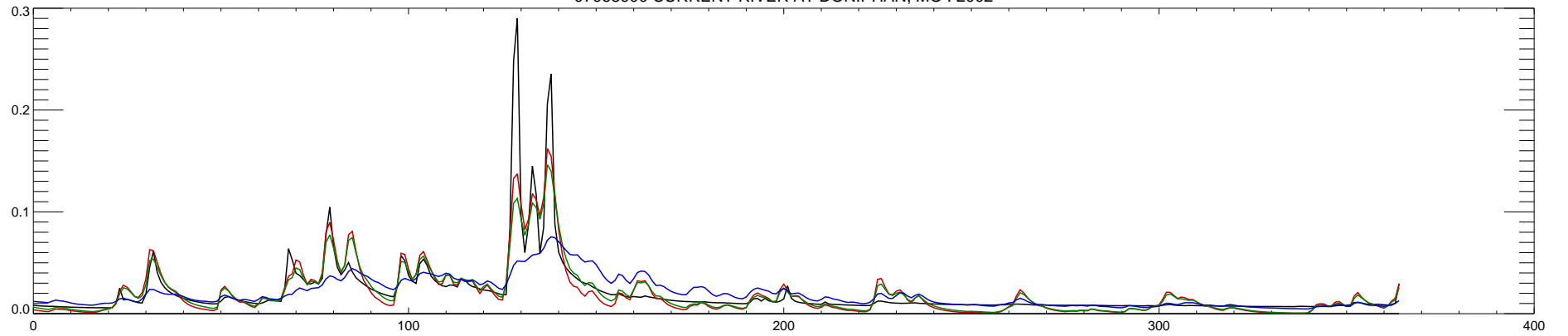
07068000 CURRENT RIVER AT DONIPHAN, MO : 2003
