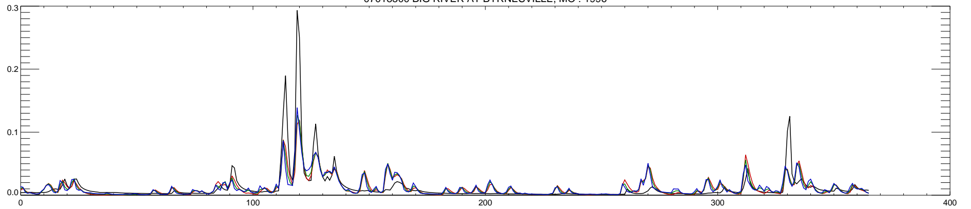
07018500 BIG RIVER AT BYRNESVILLE, MO : 1997
