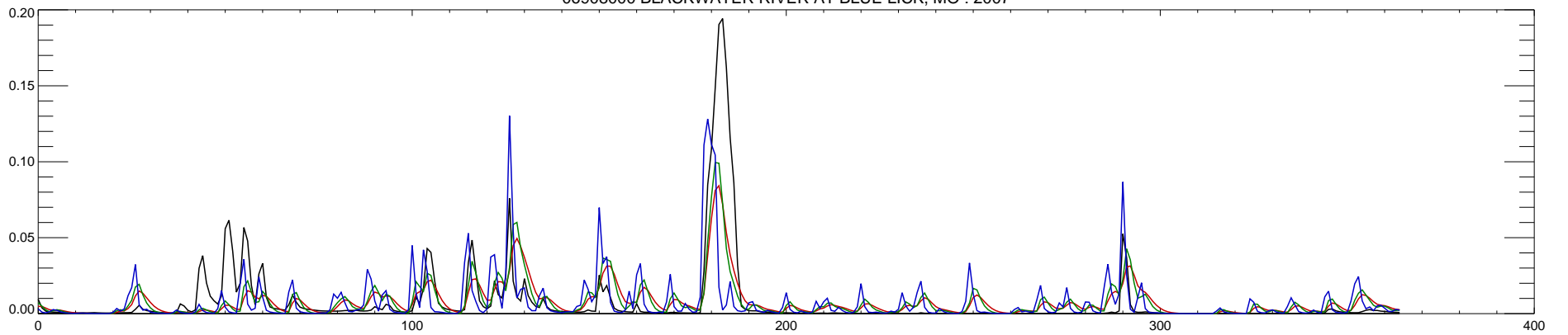
06908000 BLACKWATER RIVER AT BLUE LICK, MO : 2007
