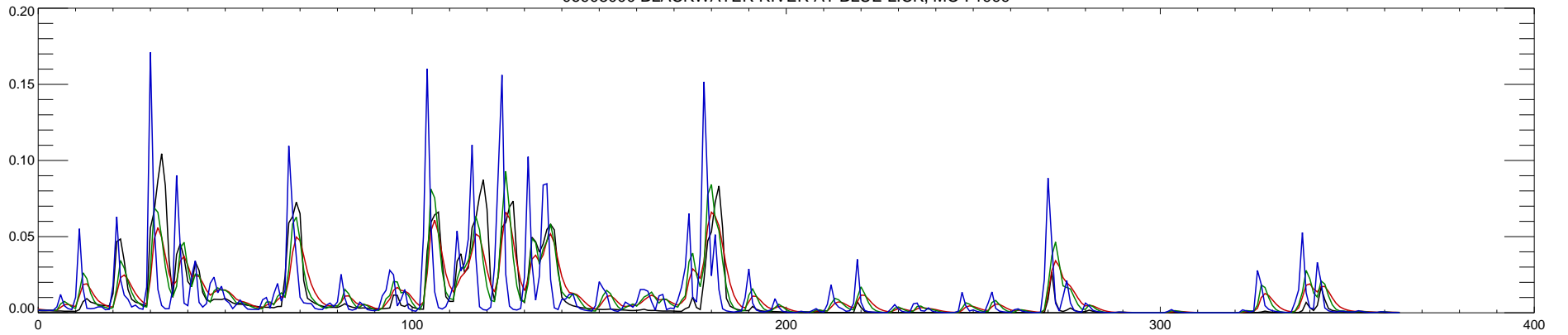
06908000 BLACKWATER RIVER AT BLUE LICK, MO : 2000
