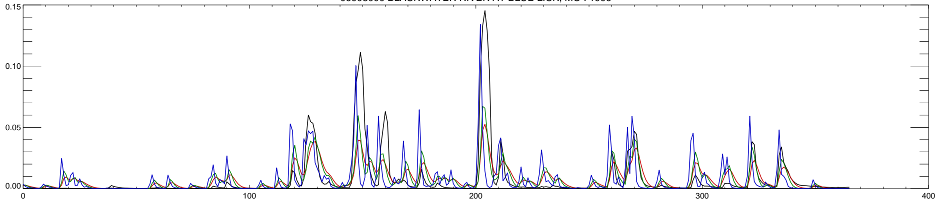
06908000 BLACKWATER RIVER AT BLUE LICK, MO : 1997
