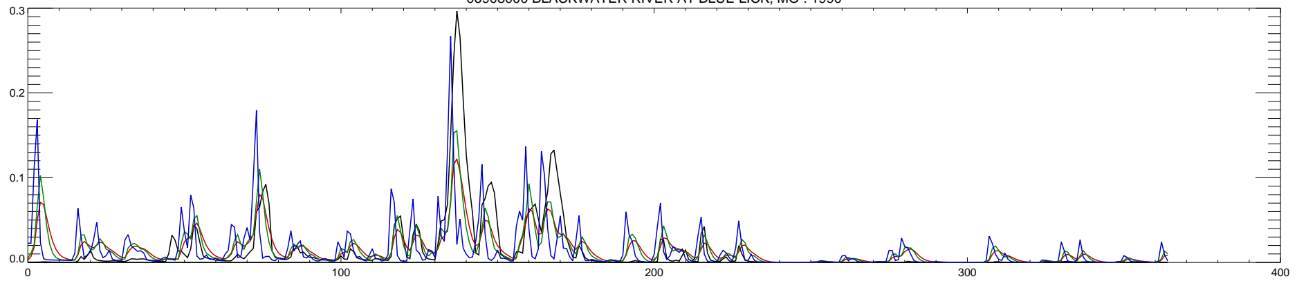
06908000 BLACKWATER RIVER AT BLUE LICK, MO : 1991
