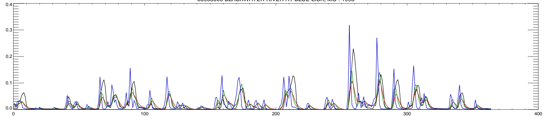
06908000 BLACKWATER RIVER AT BLUE LICK, MO : 1998
