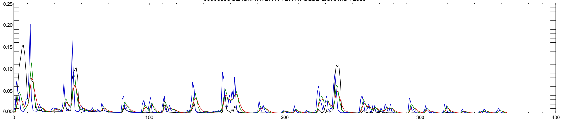
06908000 BLACKWATER RIVER AT BLUE LICK, MO : 2006
