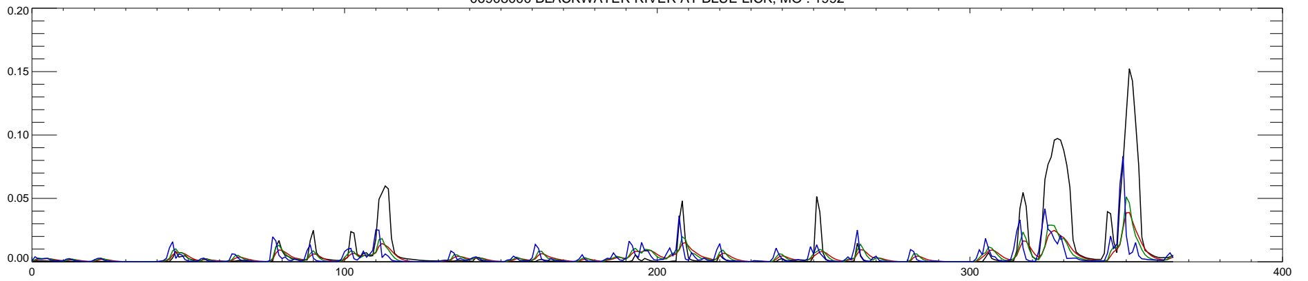
06908000 BLACKWATER RIVER AT BLUE LICK, MO : 1992
