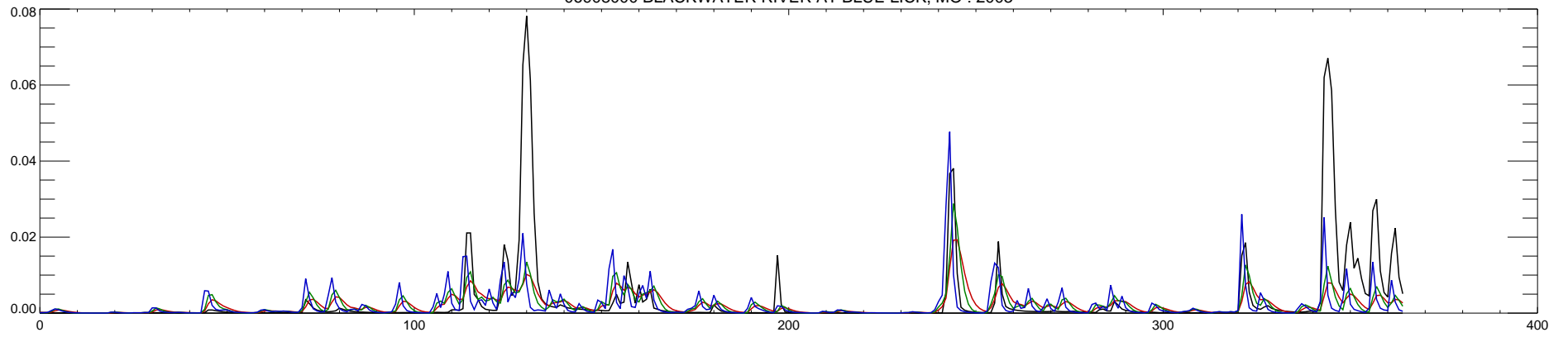
06908000 BLACKWATER RIVER AT BLUE LICK, MO : 2004
