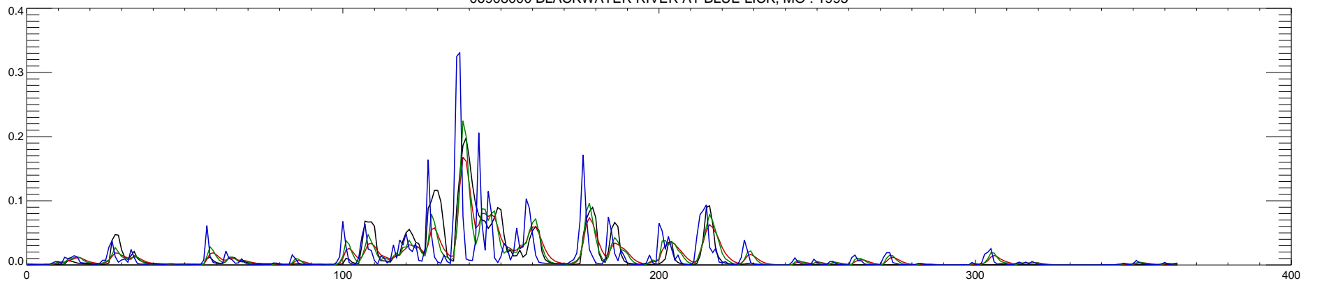
06908000 BLACKWATER RIVER AT BLUE LICK, MO : 1995
