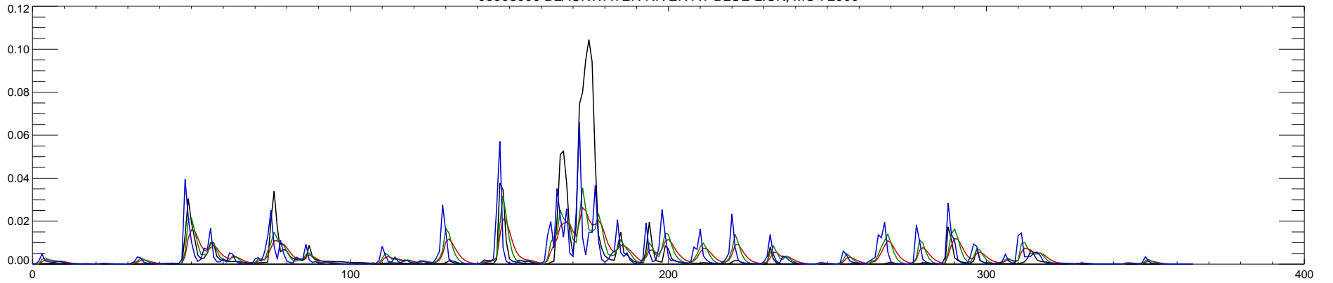
06908000 BLACKWATER RIVER AT BLUE LICK, MO : 2001
