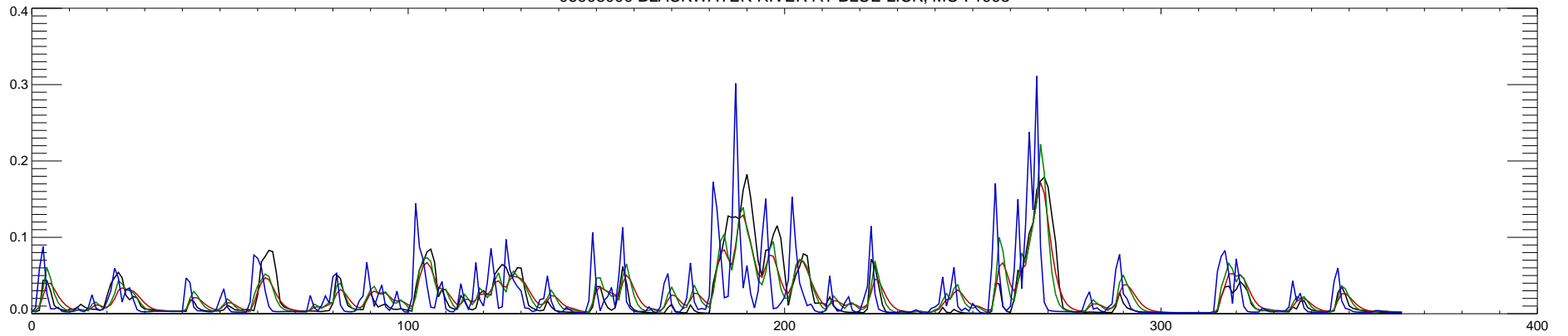
06908000 BLACKWATER RIVER AT BLUE LICK, MO : 1994
