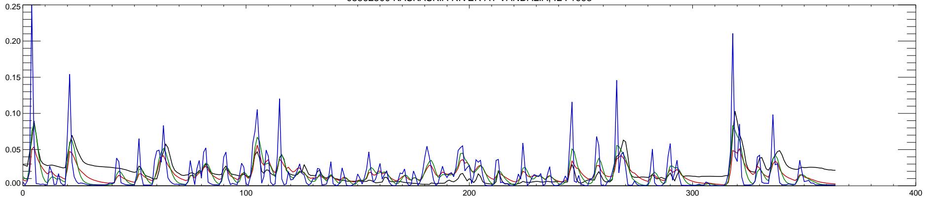
05592500 KASKASKIA RIVER AT VANDALIA, IL : 1994
