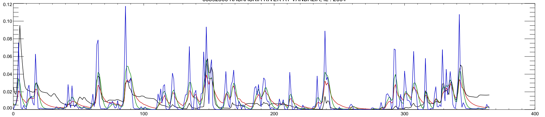
05592500 KASKASKIA RIVER AT VANDALIA, IL : 2004
