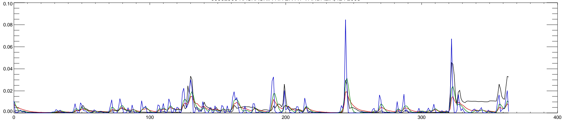
05592500 KASKASKIA RIVER AT VANDALIA, IL : 2004
