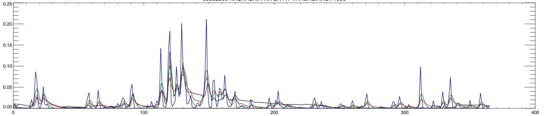
05592500 KASKASKIA RIVER AT VANDALIA, IL : 1997
