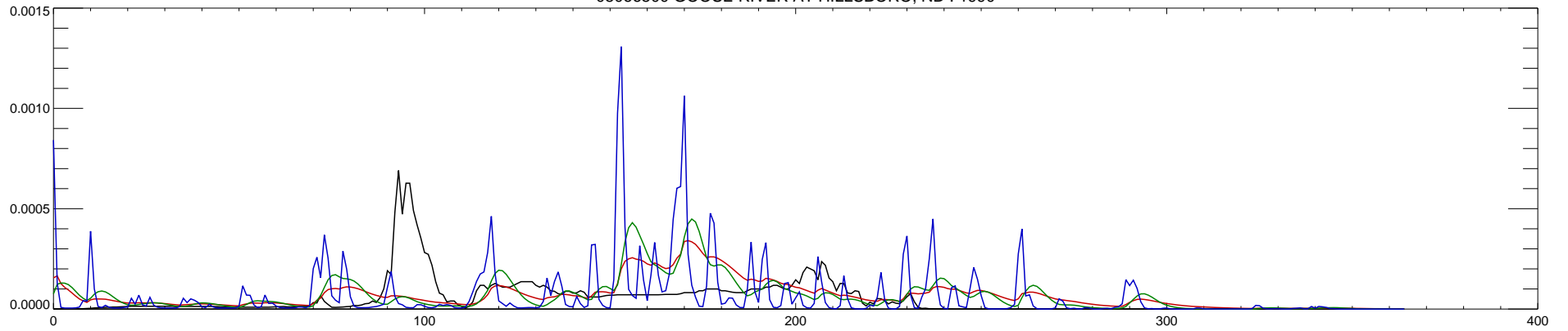
05066500 GOOSE RIVER AT HILLSBORO, ND : 1991
