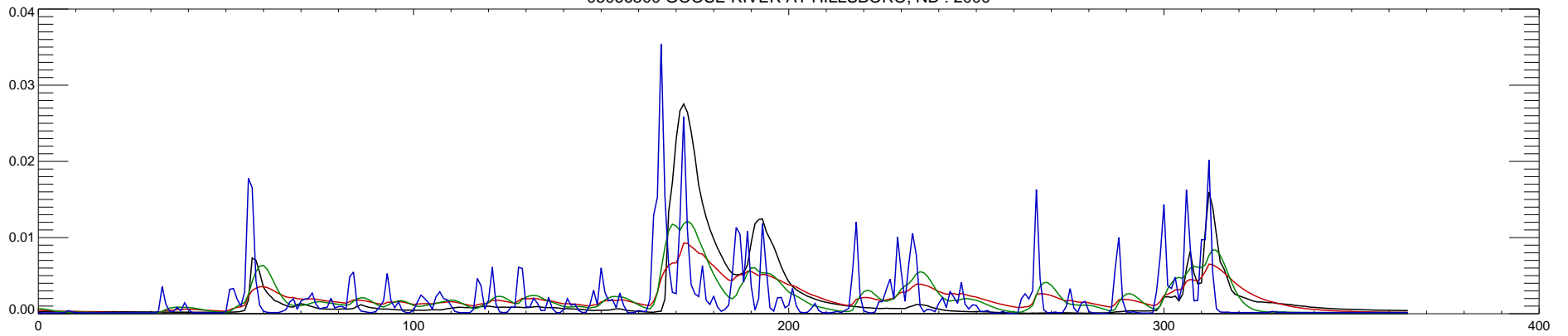
05066500 GOOSE RIVER AT HILLSBORO, ND : 2001
