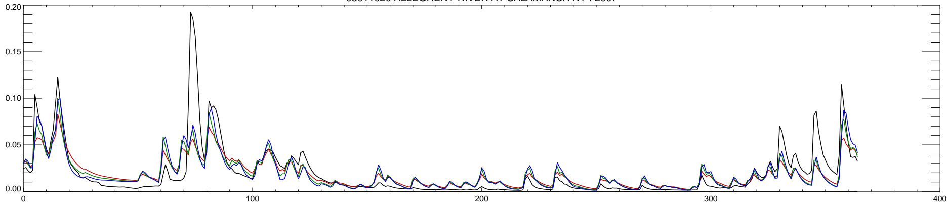
03011020 ALLEGHENY RIVER AT SALAMANCA NY : 2007
