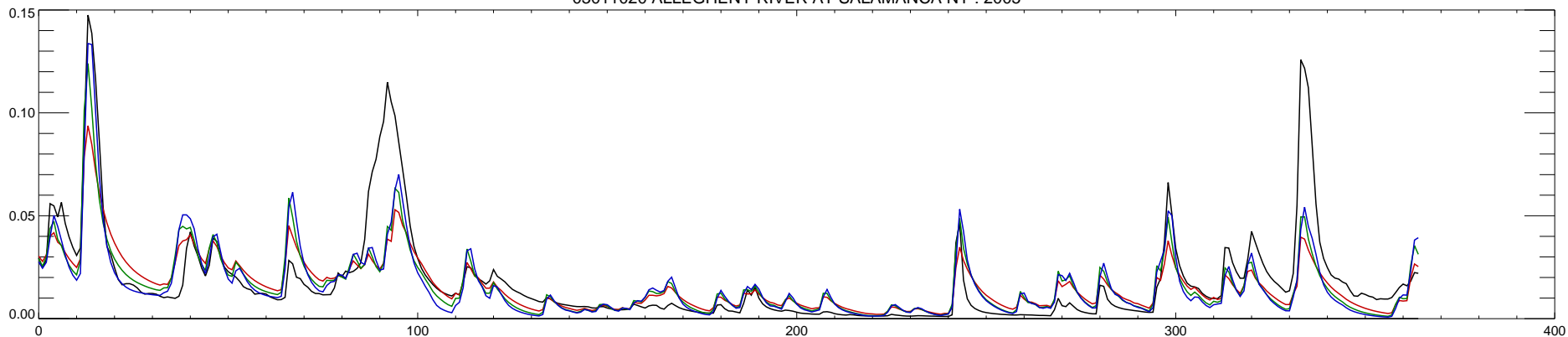
03011020 ALLEGHENY RIVER AT SALAMANCA NY : 2006
