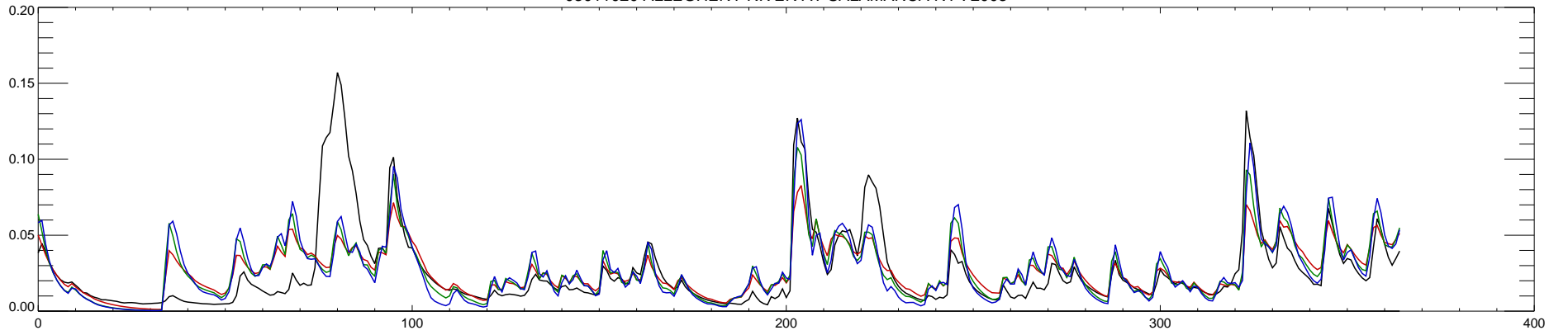
03011020 ALLEGHENY RIVER AT SALAMANCA NY : 2004
