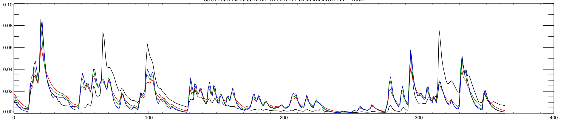
03011020 ALLEGHENY RIVER AT SALAMANCA NY : 1995
