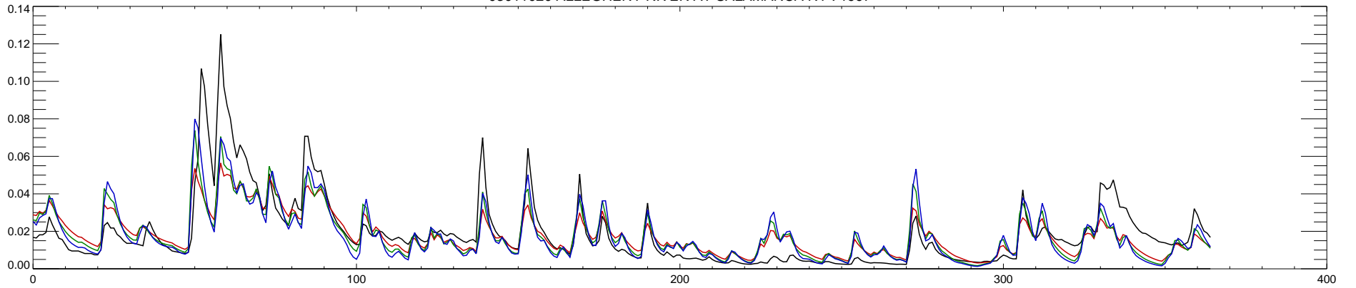
03011020 ALLEGHENY RIVER AT SALAMANCA NY : 1998
