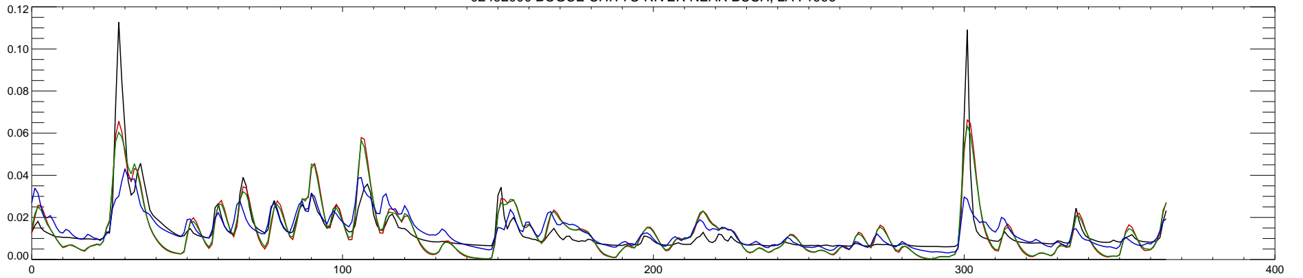
02492000 BOGUE CHITTO RIVER NEAR BUSH, LA : 1997
