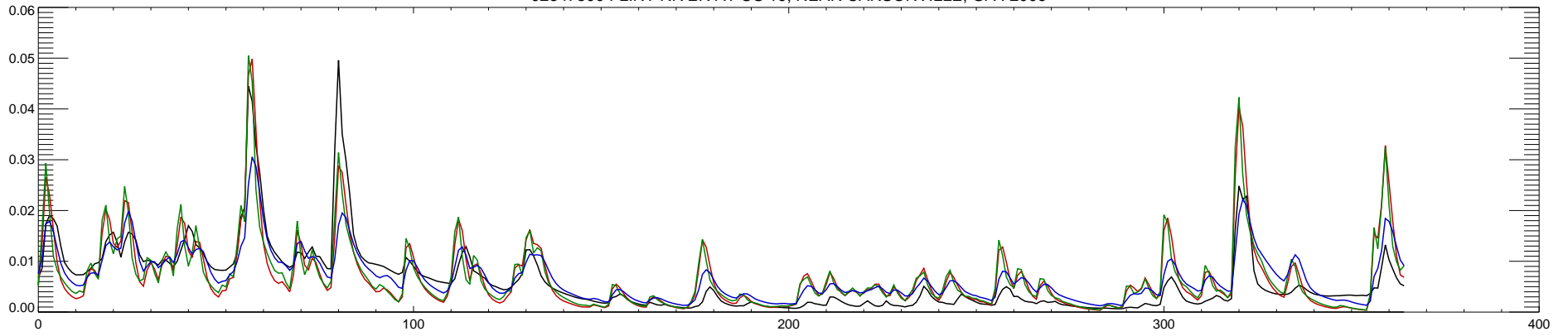
02347500 FLINT RIVER AT US 19, NEAR CARSONVILLE, GA : 2007
