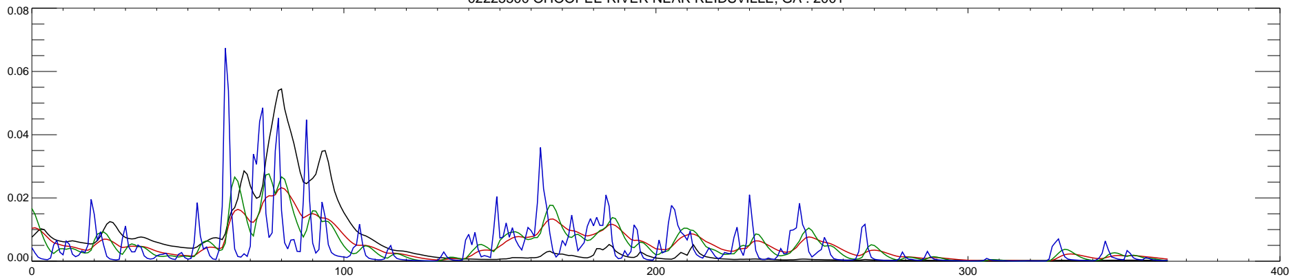
02225500 OHOOPEE RIVER NEAR REIDSVILLE, GA : 2001
