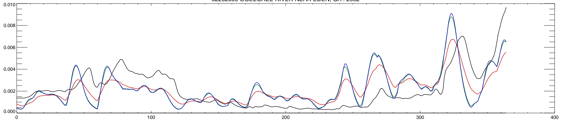
02202500 OGEECHEE RIVER NEAR EDEN, GA : 2003
