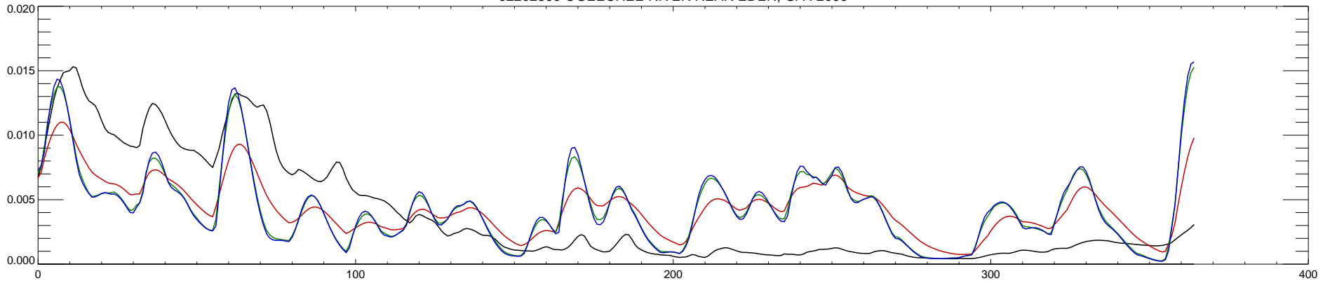
02202500 OGEECHEE RIVER NEAR EDEN, GA : 2007
