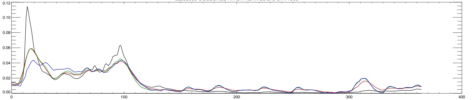
02202500 OGEECHEE RIVER NEAR EDEN, GA : 1994
