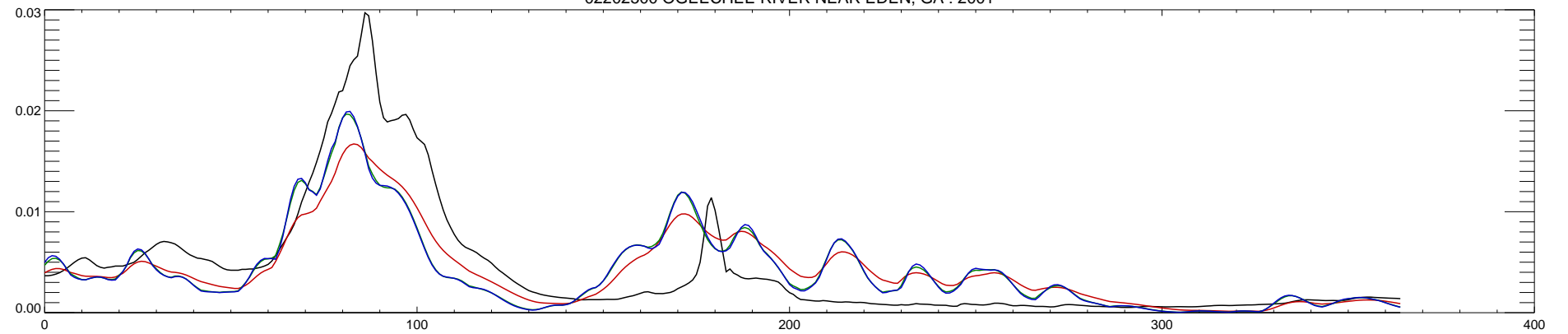
02202500 OGEECHEE RIVER NEAR EDEN, GA : 2001
