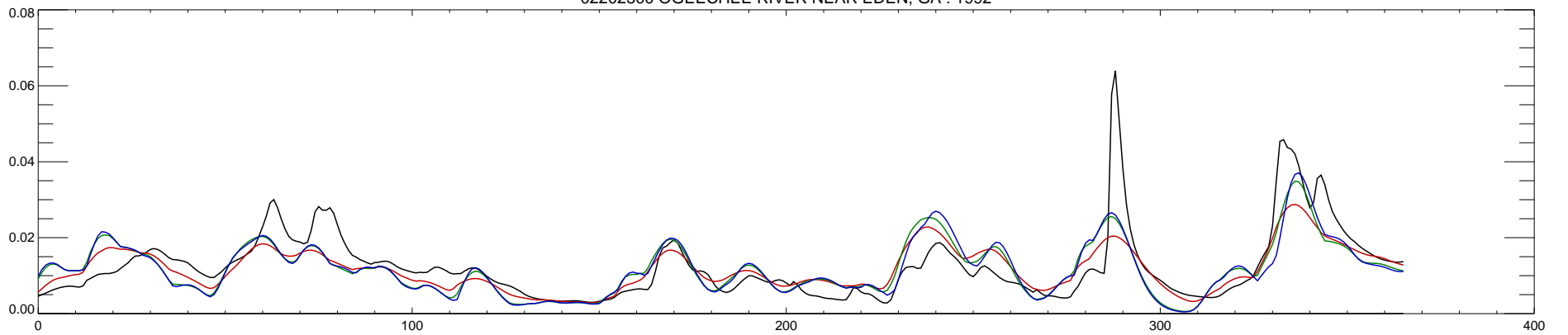
02202500 OGEECHEE RIVER NEAR EDEN, GA : 1992
