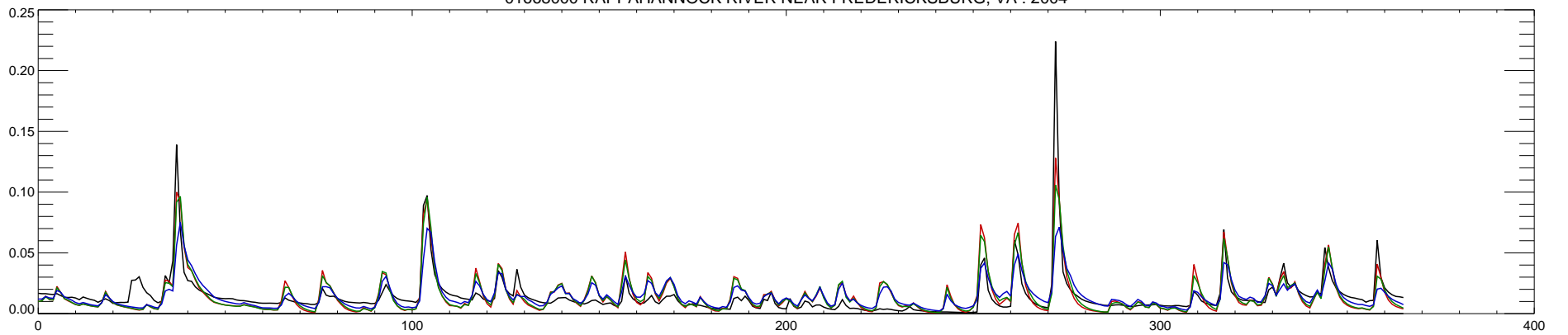
01668000 RAPPAHANNOCK RIVER NEAR FREDERICKSBURG, VA : 2004
