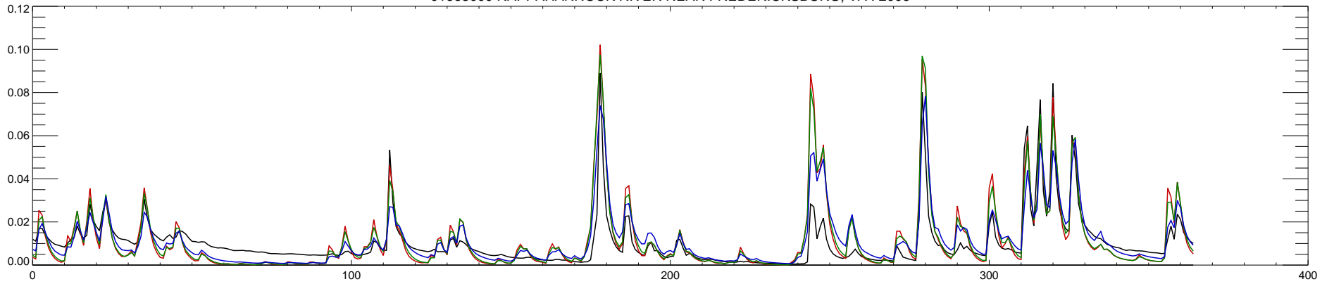
01668000 RAPPAHANNOCK RIVER NEAR FREDERICKSBURG, VA : 2007
