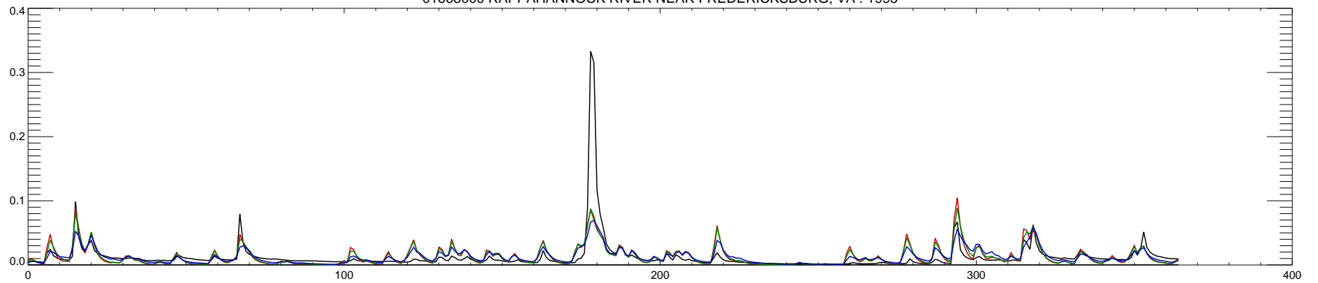
01668000 RAPPAHANNOCK RIVER NEAR FREDERICKSBURG, VA : 1995
