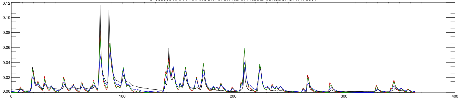
01668000 RAPPAHANNOCK RIVER NEAR FREDERICKSBURG, VA : 2001
