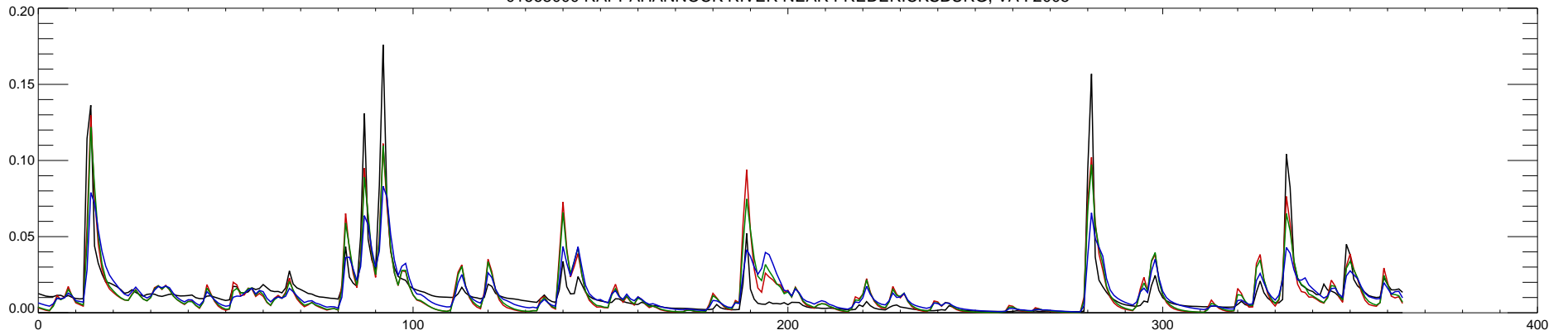
01668000 RAPPAHANNOCK RIVER NEAR FREDERICKSBURG, VA : 2006
