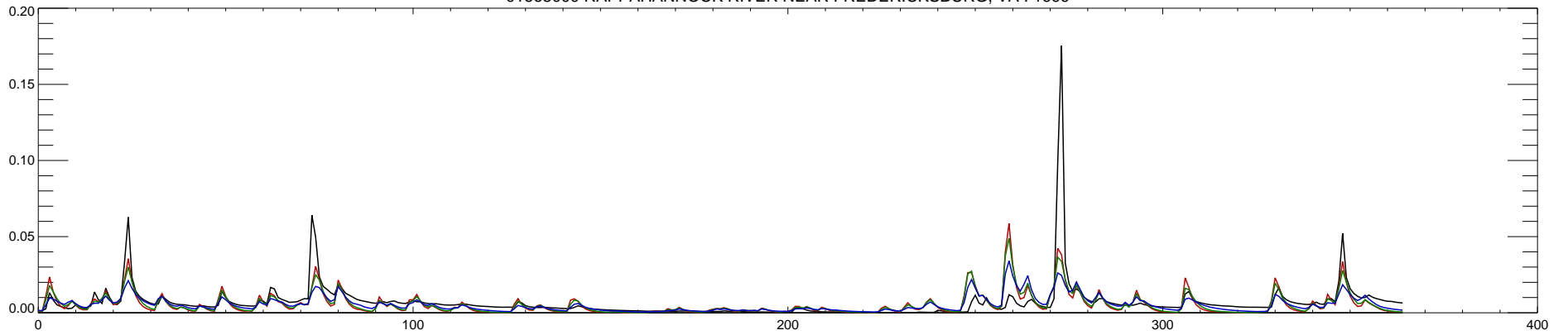
01668000 RAPPAHANNOCK RIVER NEAR FREDERICKSBURG, VA : 2000
