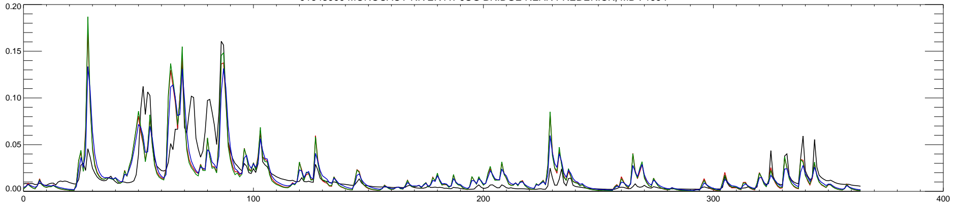
01643000 MONOCACY RIVER AT JUG BRIDGE NEAR FREDERICK, MD : 1995
