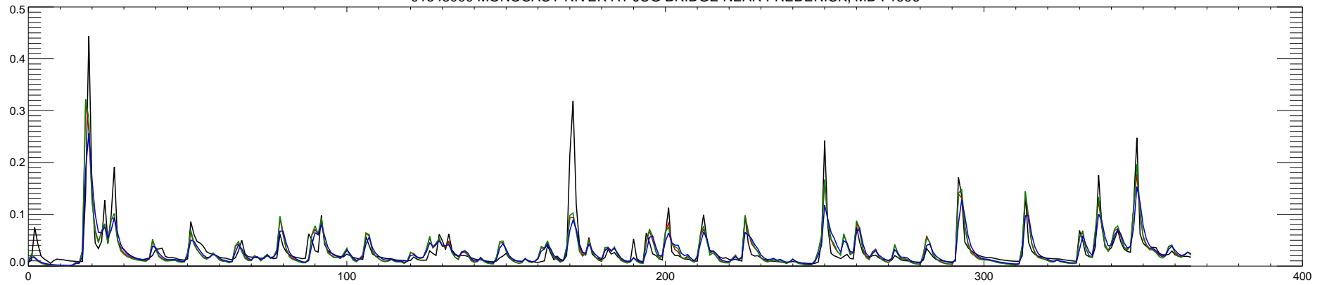
01643000 MONOCACY RIVER AT JUG BRIDGE NEAR FREDERICK, MD : 1997
