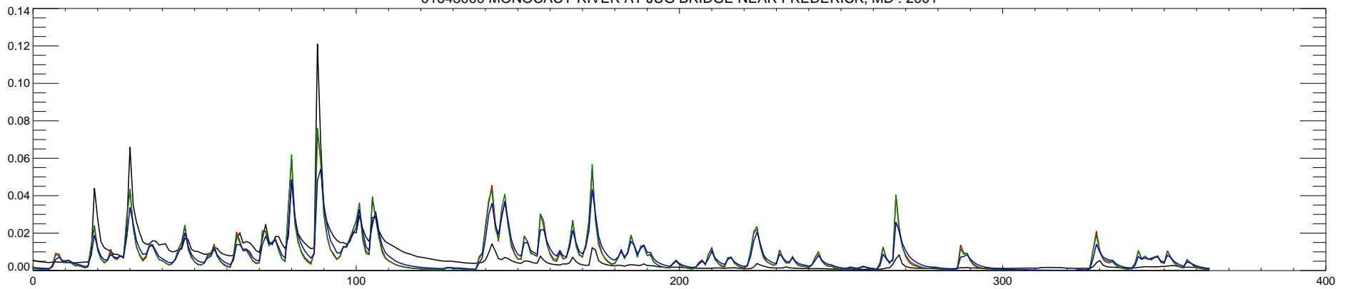
01643000 MONOCACY RIVER AT JUG BRIDGE NEAR FREDERICK, MD : 2001
