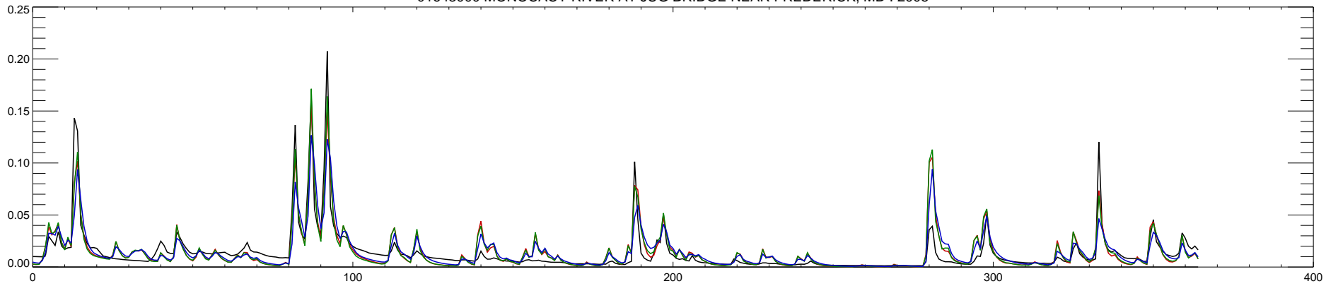
01643000 MONOCACY RIVER AT JUG BRIDGE NEAR FREDERICK, MD : 2006
