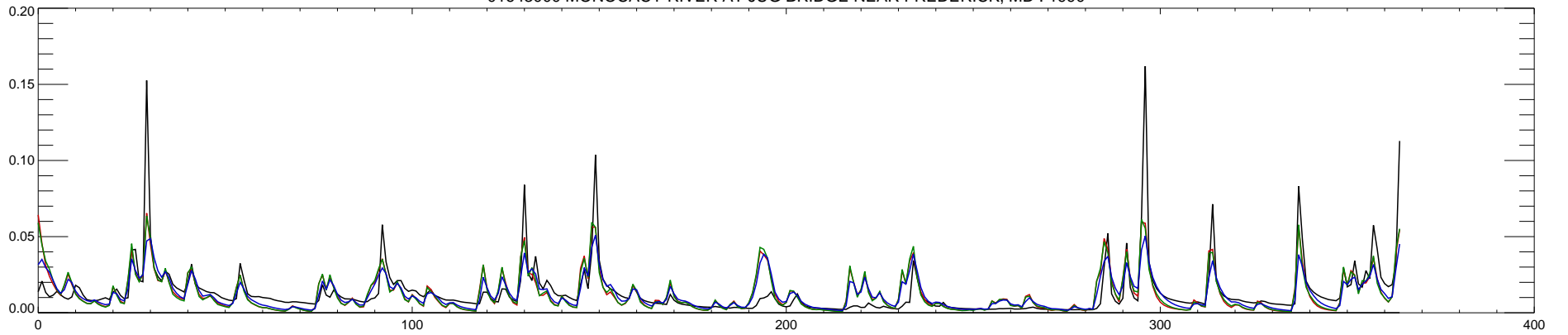
01643000 MONOCACY RIVER AT JUG BRIDGE NEAR FREDERICK, MD : 1991
