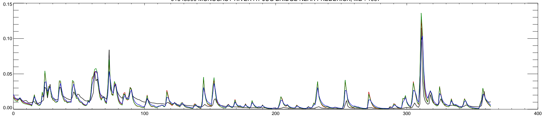
01643000 MONOCACY RIVER AT JUG BRIDGE NEAR FREDERICK, MD : 1998
