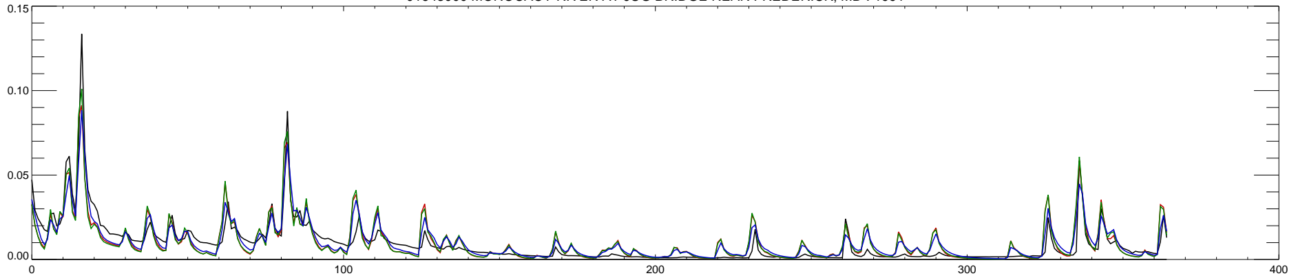
01643000 MONOCACY RIVER AT JUG BRIDGE NEAR FREDERICK, MD : 1992
