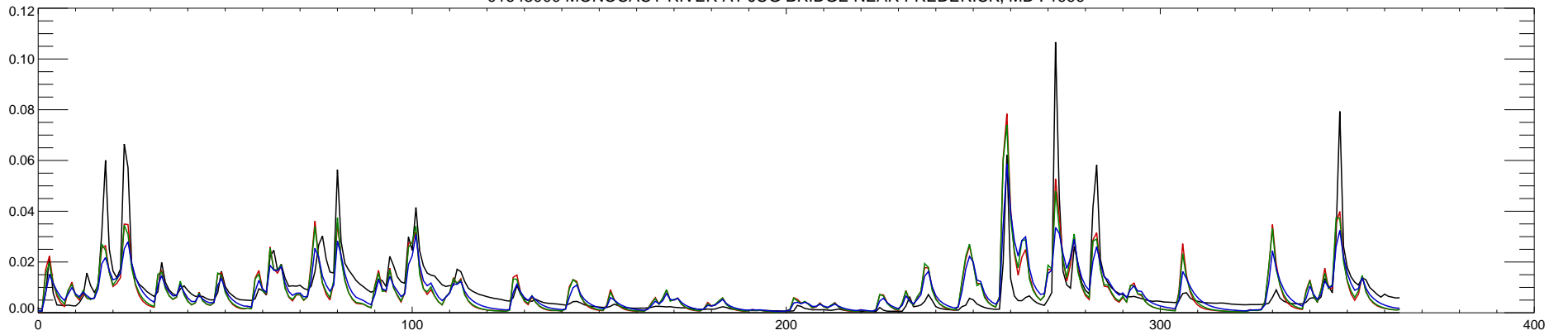
01643000 MONOCACY RIVER AT JUG BRIDGE NEAR FREDERICK, MD : 2000
