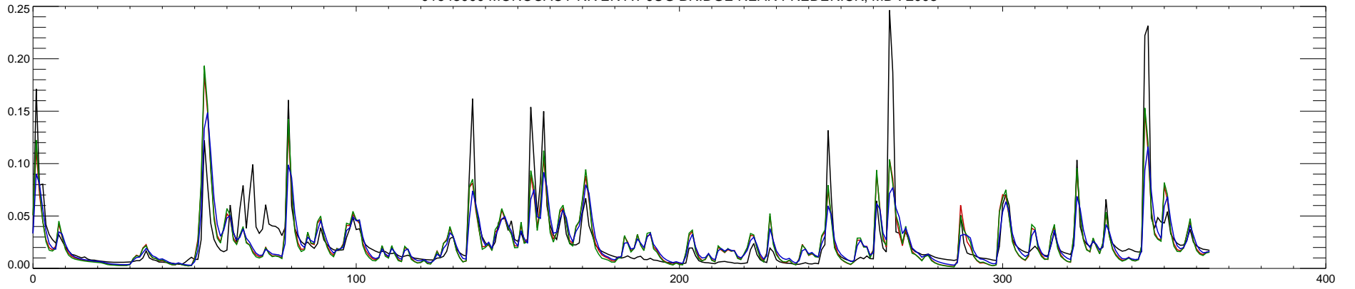
01643000 MONOCACY RIVER AT JUG BRIDGE NEAR FREDERICK, MD : 2004
