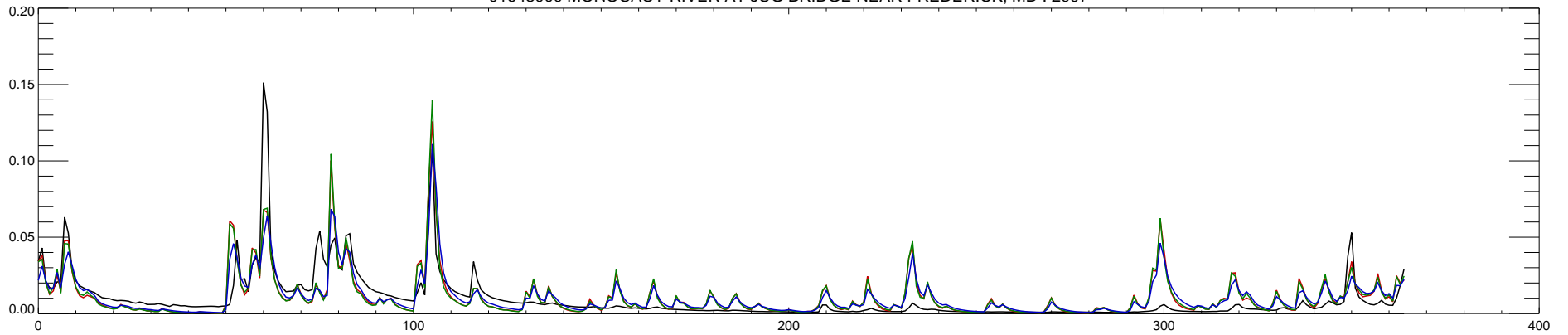
01643000 MONOCACY RIVER AT JUG BRIDGE NEAR FREDERICK, MD : 2007
