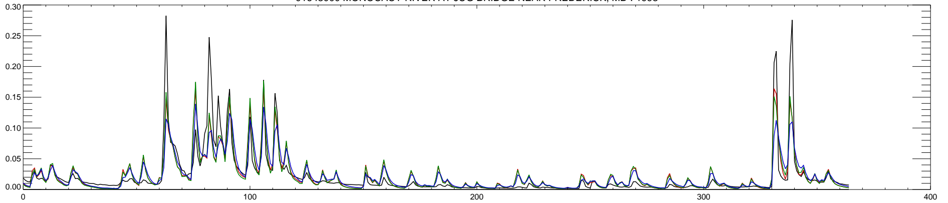
01643000 MONOCACY RIVER AT JUG BRIDGE NEAR FREDERICK, MD : 1994
