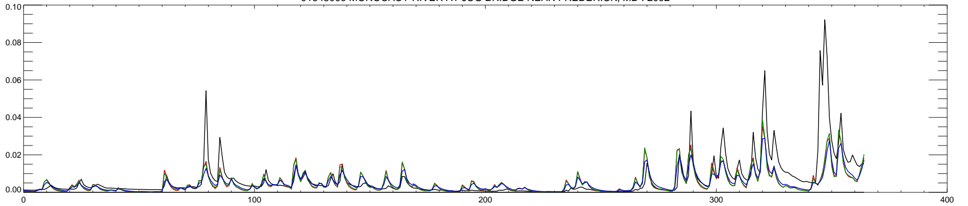
01643000 MONOCACY RIVER AT JUG BRIDGE NEAR FREDERICK, MD : 2003
