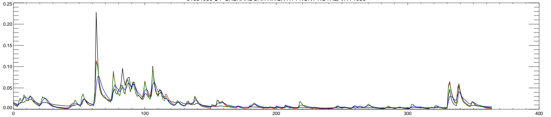
01631000 S F SHENANDOAH RIVER AT FRONT ROYAL, VA : 1994
