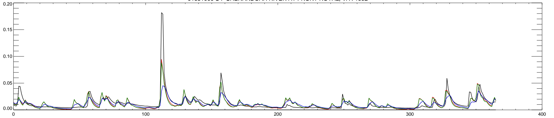
01631000 S F SHENANDOAH RIVER AT FRONT ROYAL, VA : 1992
