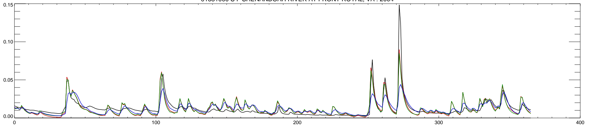
01631000 S F SHENANDOAH RIVER AT FRONT ROYAL, VA : 2004
