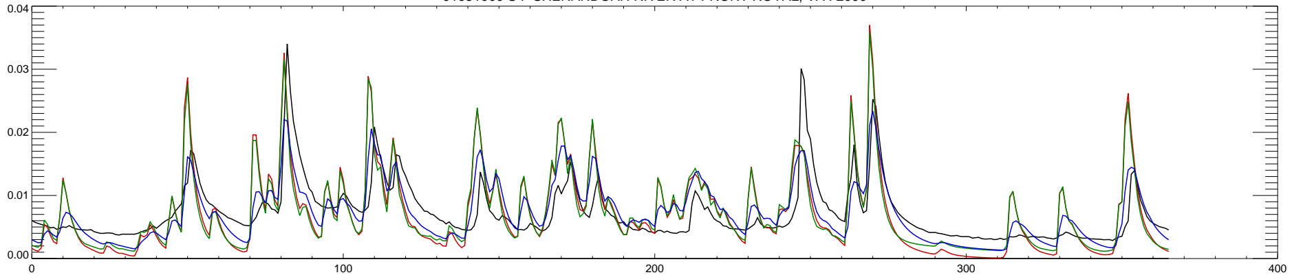
01631000 S F SHENANDOAH RIVER AT FRONT ROYAL, VA : 2001
