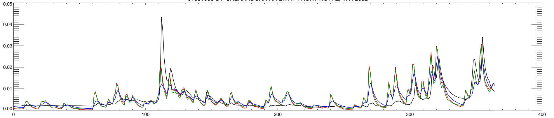
01631000 S F SHENANDOAH RIVER AT FRONT ROYAL, VA : 2003
