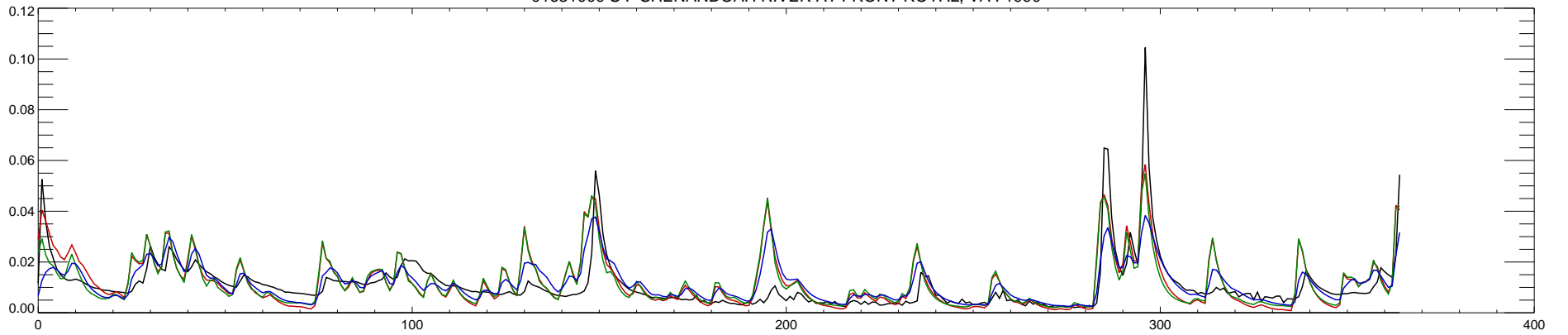
01631000 S F SHENANDOAH RIVER AT FRONT ROYAL, VA : 1991
