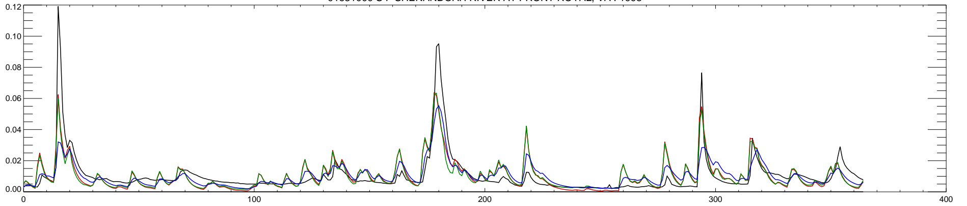
01631000 S F SHENANDOAH RIVER AT FRONT ROYAL, VA : 1995
