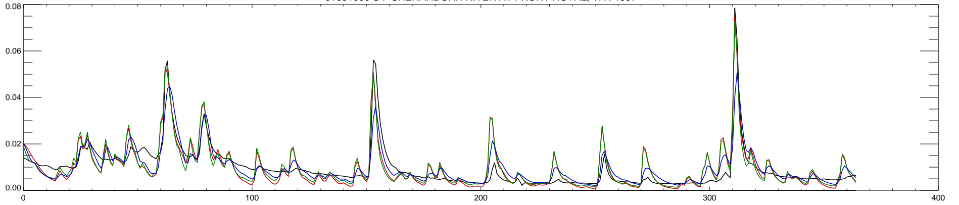
01631000 S F SHENANDOAH RIVER AT FRONT ROYAL, VA : 1998
