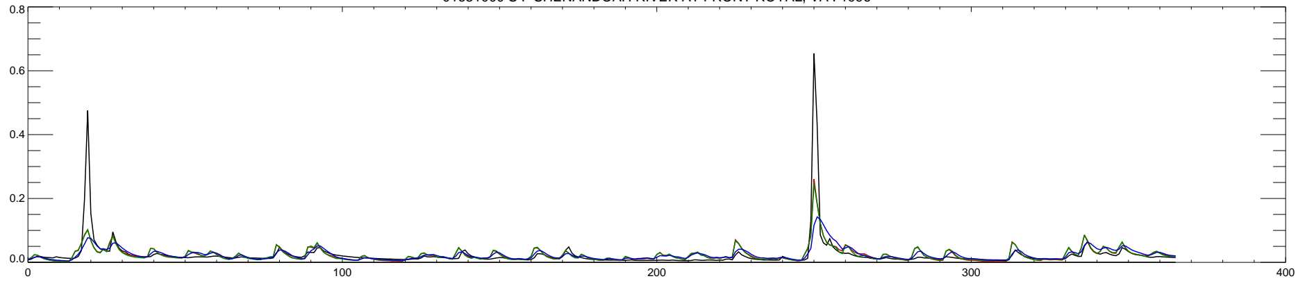
01631000 S F SHENANDOAH RIVER AT FRONT ROYAL, VA : 1997
