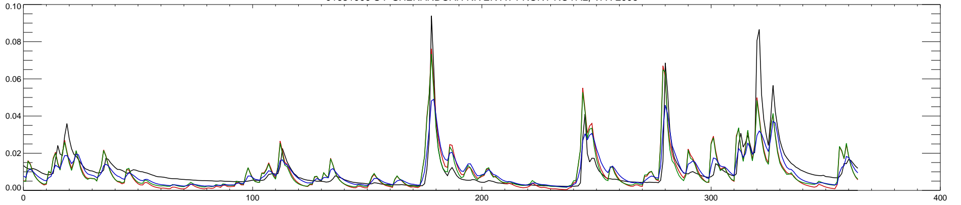
01631000 S F SHENANDOAH RIVER AT FRONT ROYAL, VA : 2007
