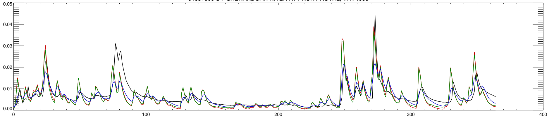
01631000 S F SHENANDOAH RIVER AT FRONT ROYAL, VA : 2000
