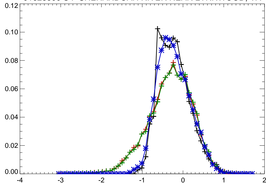
01628500 S F SHENANDOAH RIVER NEAR LYNNWOOD, VA
