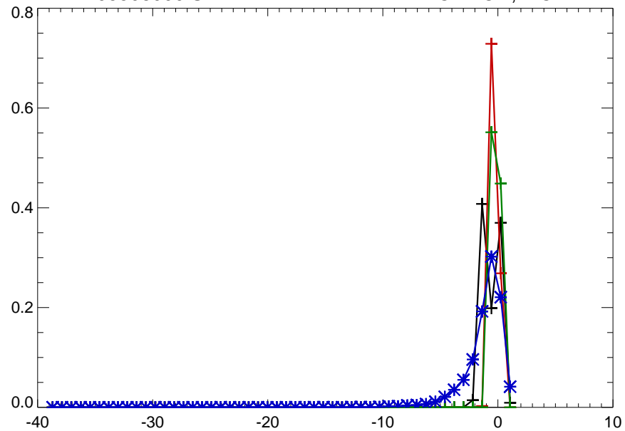
05508000 SALT RIVER NEAR NEW LONDON, MO
