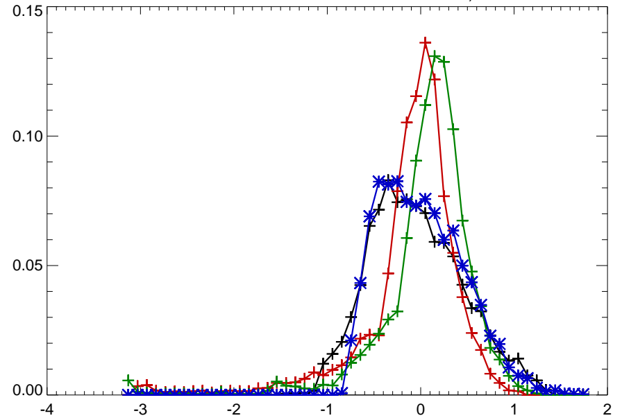
01010500 ST. JOHN RIVER AT DICKEY, MAINE
