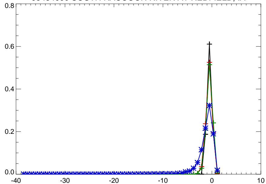
05484000 SOUTH RACCOON RIVER AT REDFIELD, IA
