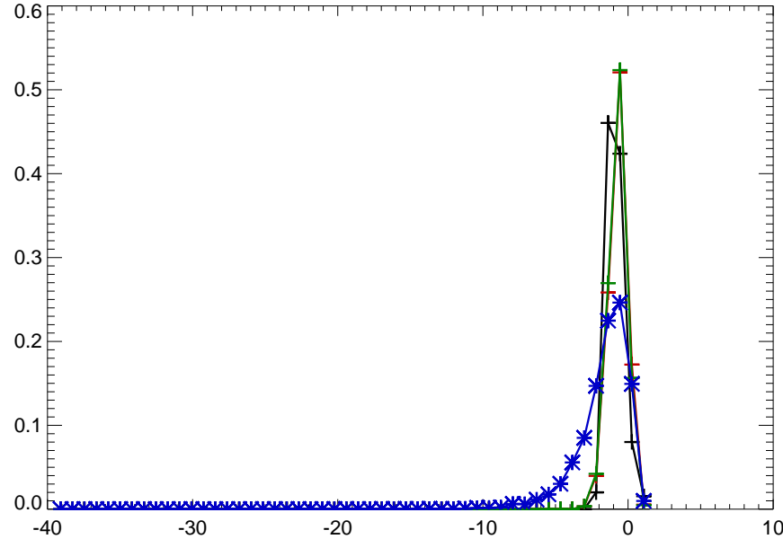
06815000 BIG NEMAHA RIVER AT FALLS CITY, NEBR.
