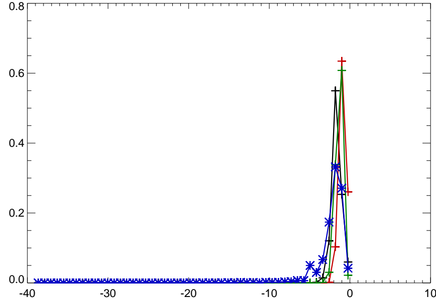
06635000 MEDICINE BOW R AB SEMINOE RESERVOIR, NR HANNA, WY
