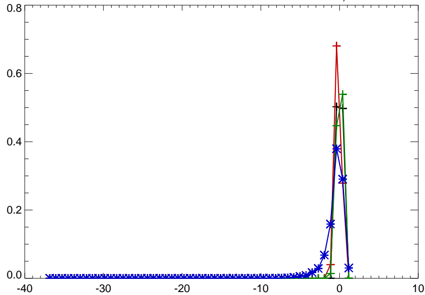
05518000 KANKAKEE RIVER AT SHELBY, IN
