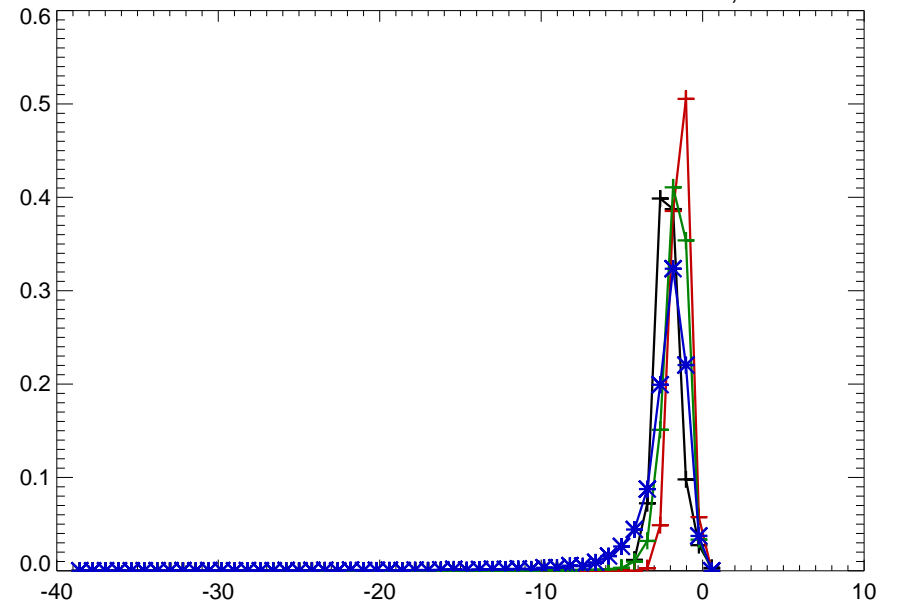
06339500 KNIFE RIVER NR GOLDEN VALLEY, ND
