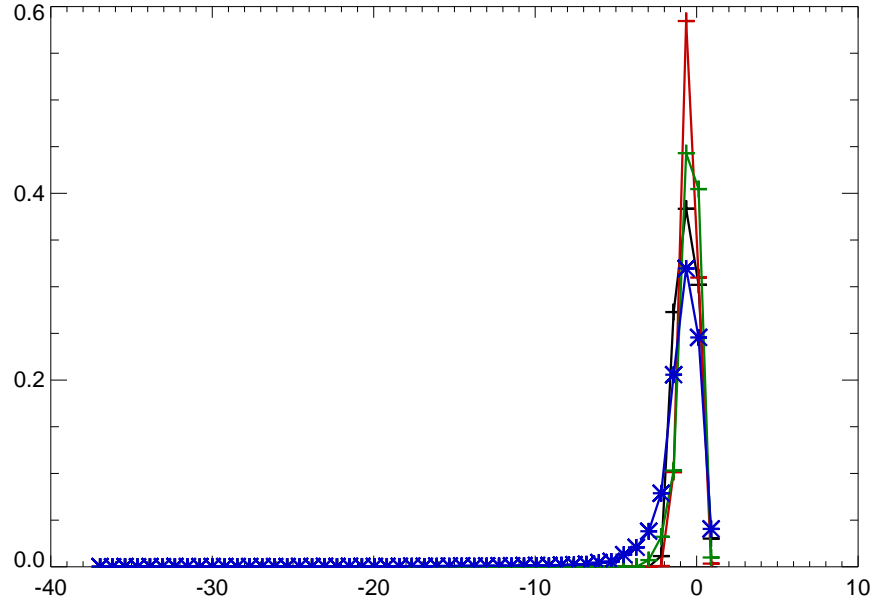
05479000 EAST FORK DES MOINES RIVER AT DAKOTA CITY, IA
