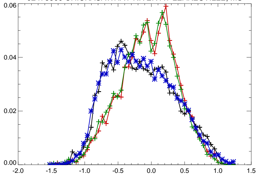
02478500 CHICKASAWHAY RIVER AT LEAKESVILLE, MS
