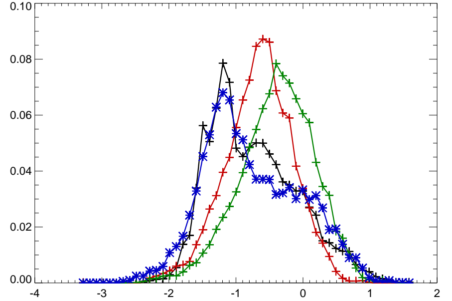
07147800 WALNUT R AT WINFIELD, KS
