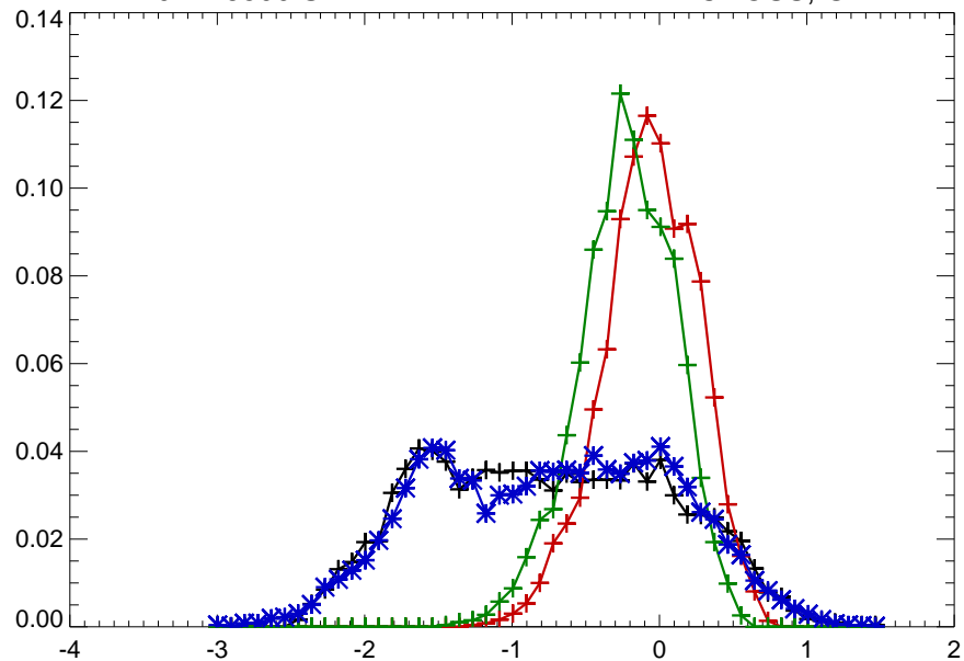
02226500 SATILLA RIVER NEAR WAYCROSS, GA
