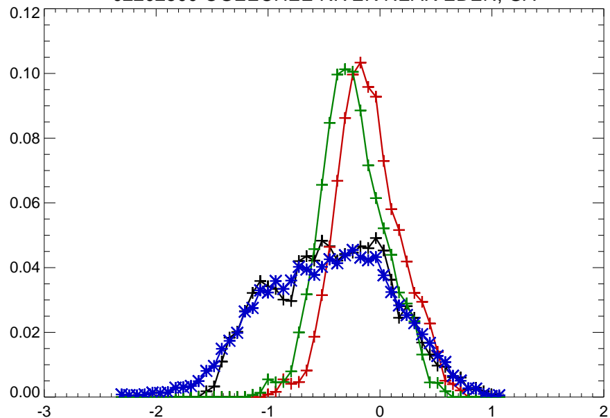
02202500 OGEECHEE RIVER NEAR EDEN, GA
