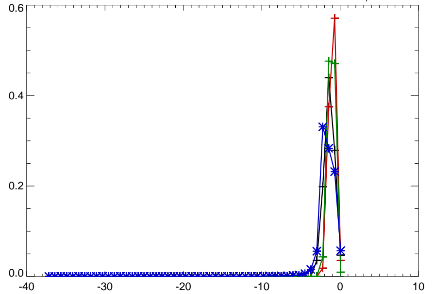
06480000 BIG SIOUX RIVER NEAR BROOKINGS, SD
