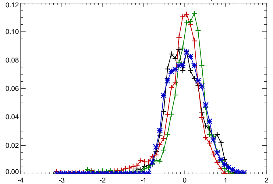
01013500 FISH RIVER NEAR FORT KENT, MAINE
