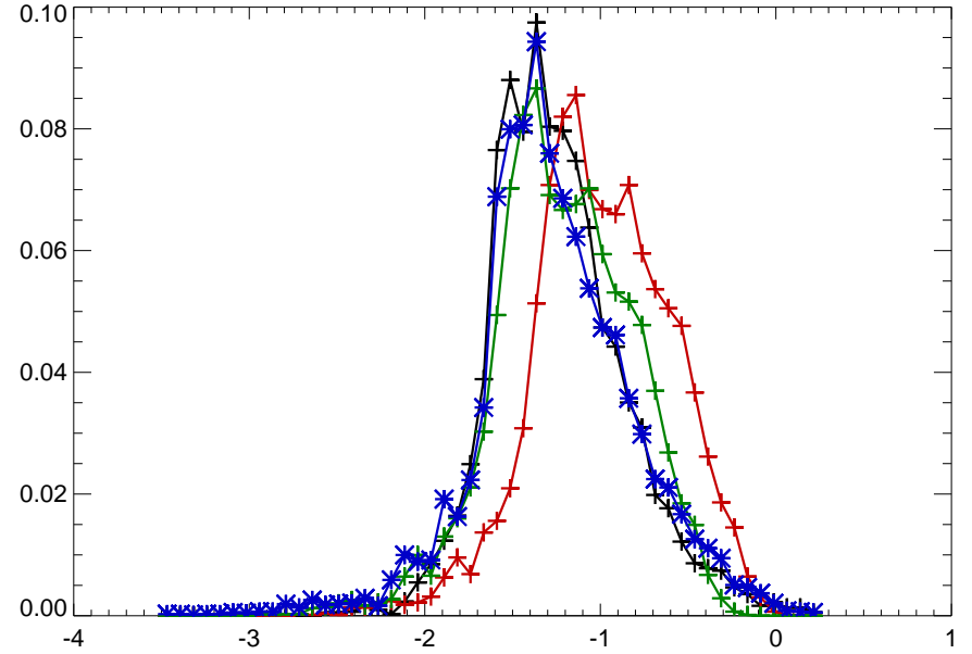
06464500 KEYA PAHA R AT WEWELA, SD
