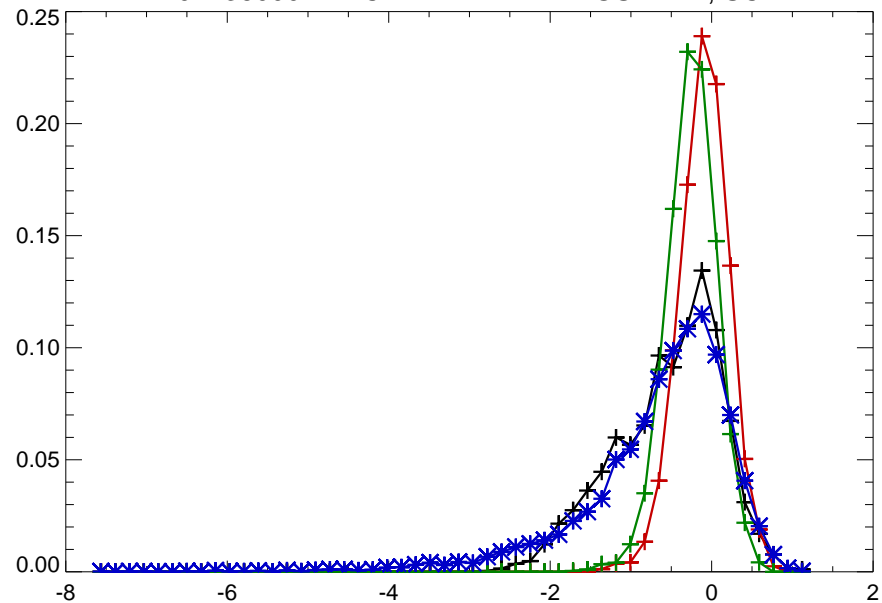
02136000 BLACK RIVER AT KINGSTREE, SC
