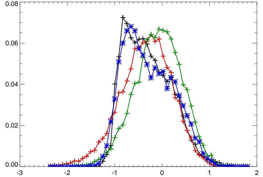
07052500 JAMES RIVER AT GALENA, MO
