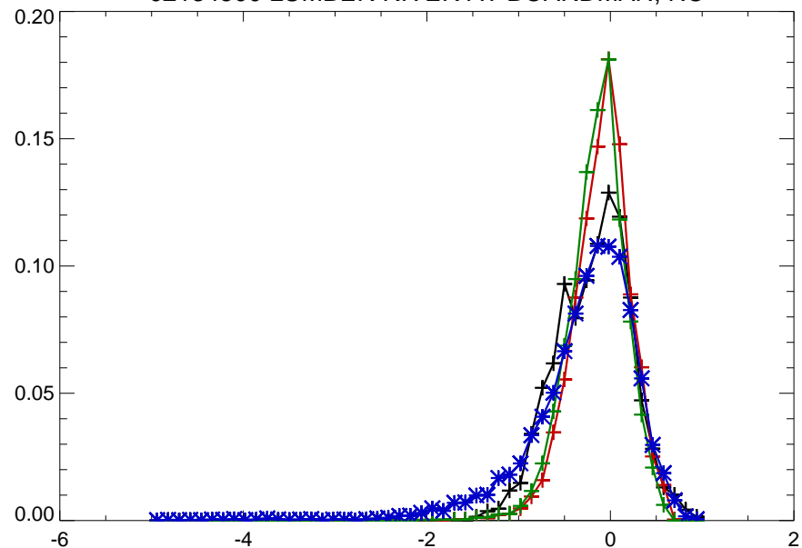
02134500 LUMBER RIVER AT BOARDMAN, NC
