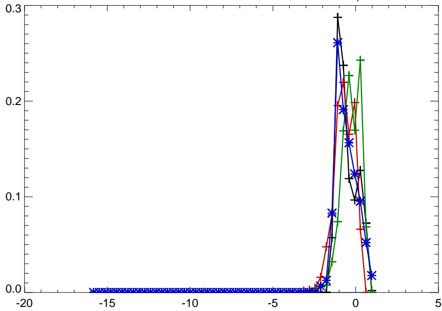
12404500 KETTLE RIVER NEAR LAURIER, WA
