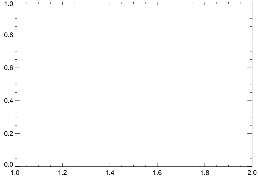
11186001 COMBINED FLOW OF KERN R AND KERN R NO 3 CA
