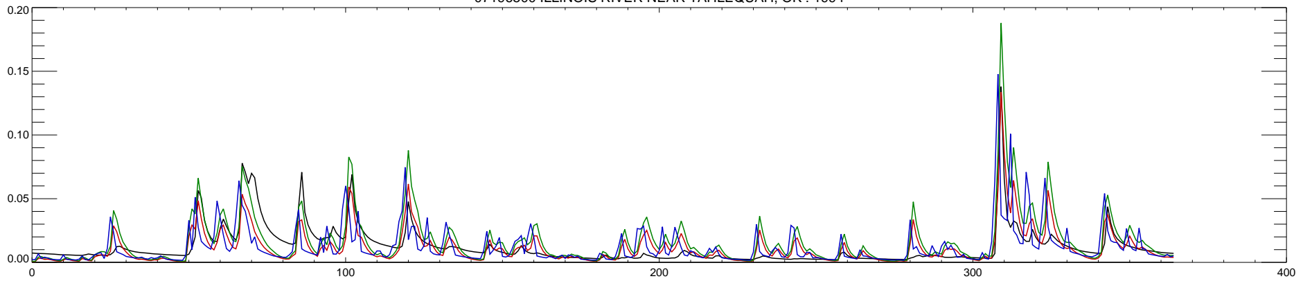
07196500 ILLINOIS RIVER NEAR TAHLEQUAH, OK : 1995
