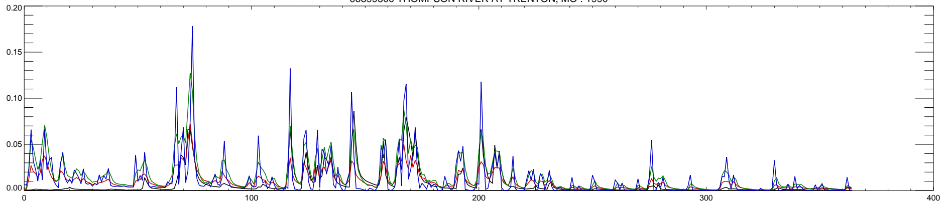
06899500 THOMPSON RIVER AT TRENTON, MO : 1991
