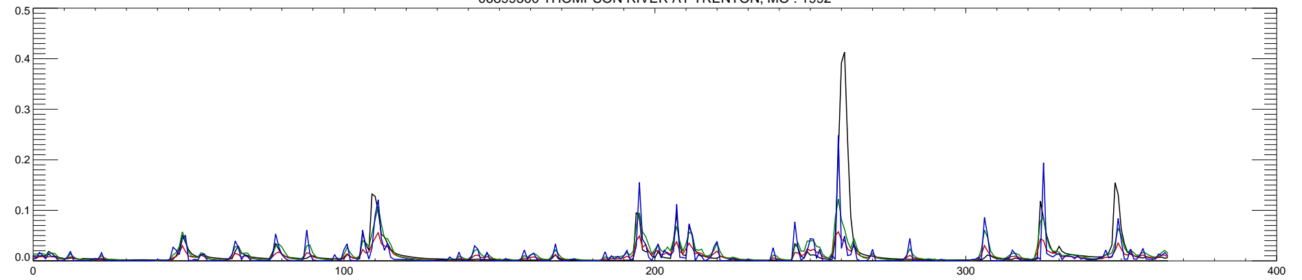
06899500 THOMPSON RIVER AT TRENTON, MO : 1992
