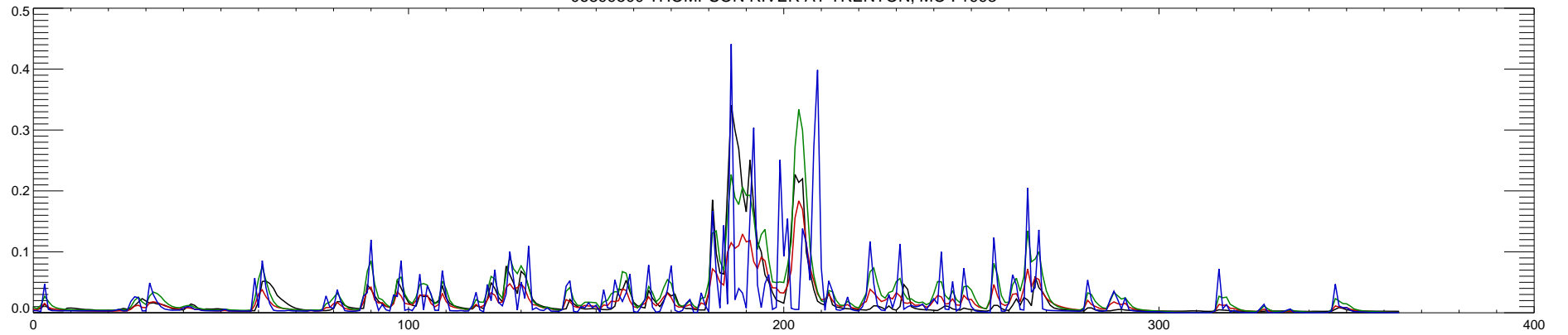
06899500 THOMPSON RIVER AT TRENTON, MO : 1994
