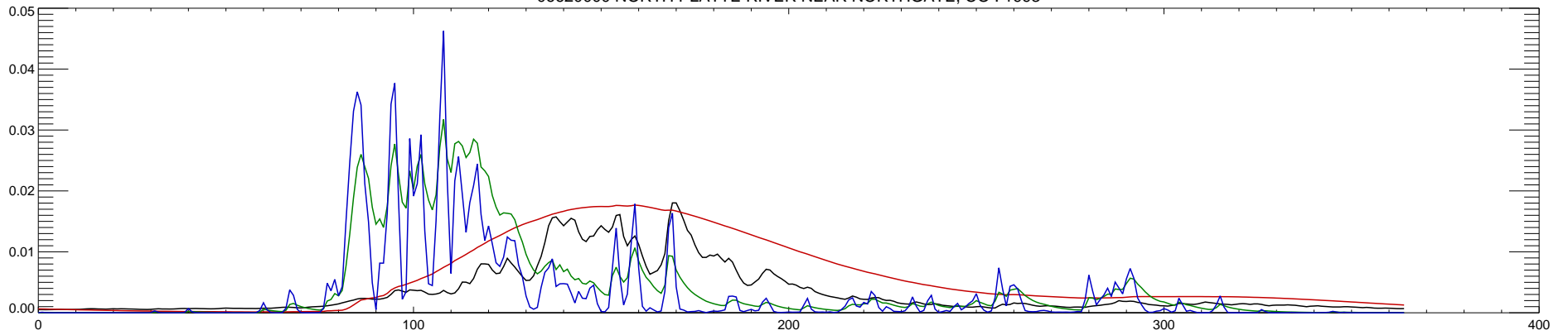
06620000 NORTH PLATTE RIVER NEAR NORTHGATE, CO : 1994
