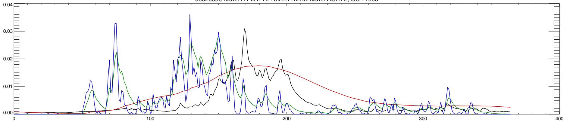
06620000 NORTH PLATTE RIVER NEAR NORTHGATE, CO : 1995
