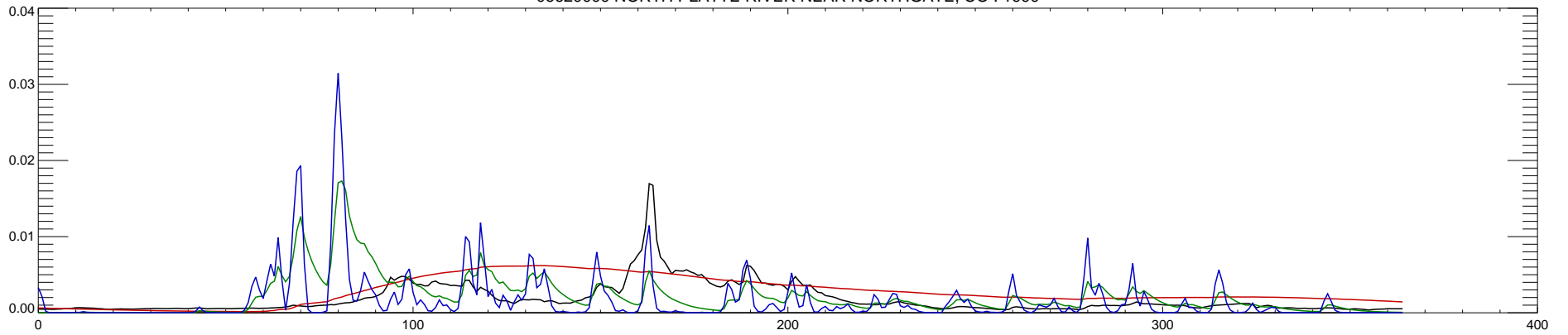
06620000 NORTH PLATTE RIVER NEAR NORTHGATE, CO : 1991
