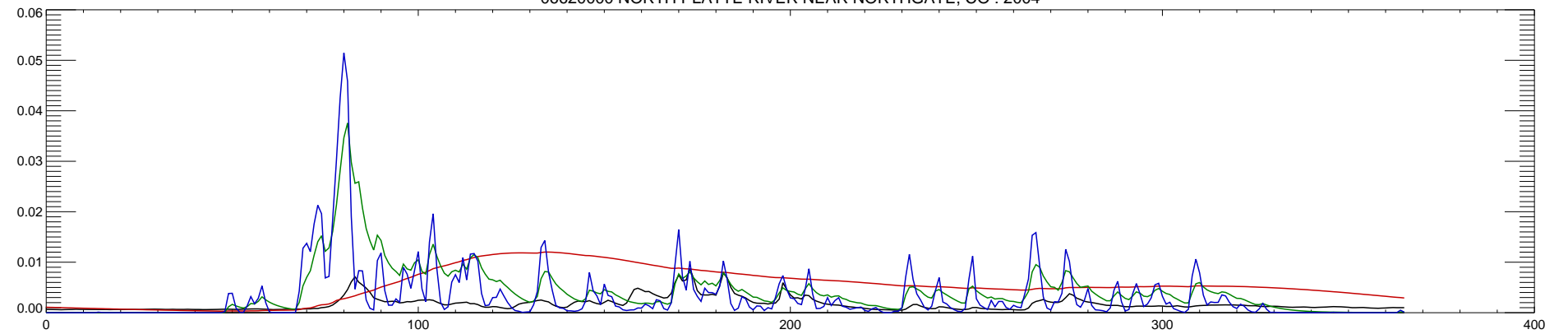
06620000 NORTH PLATTE RIVER NEAR NORTHGATE, CO : 2004
