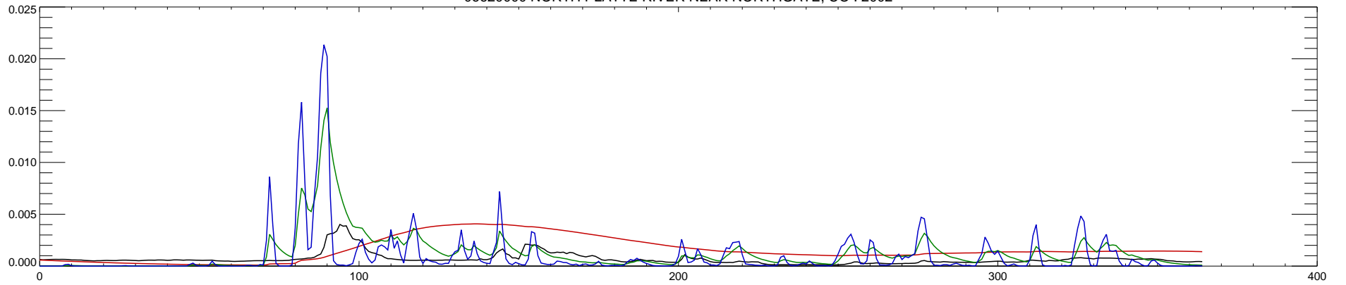
06620000 NORTH PLATTE RIVER NEAR NORTHGATE, CO : 2003
