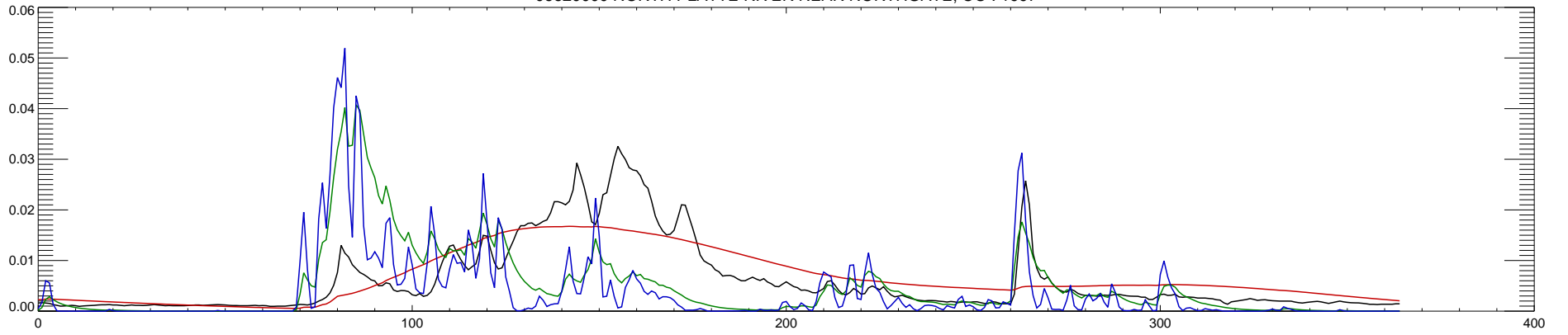
06620000 NORTH PLATTE RIVER NEAR NORTHGATE, CO : 1998
