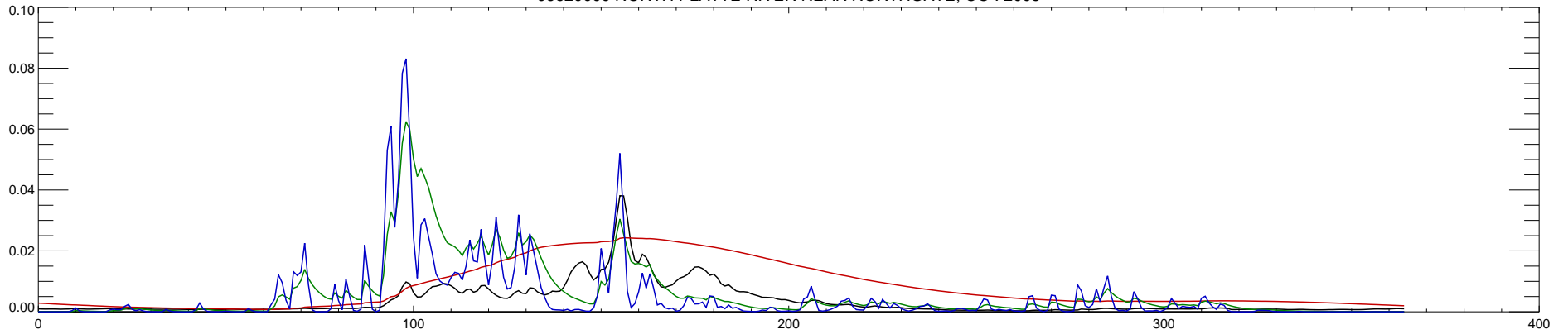
06620000 NORTH PLATTE RIVER NEAR NORTHGATE, CO : 2006
