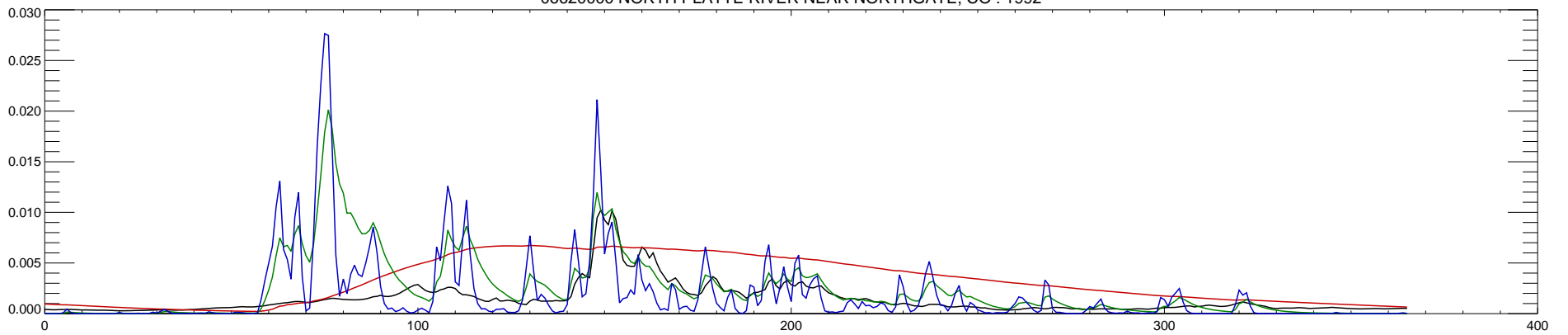
06620000 NORTH PLATTE RIVER NEAR NORTHGATE, CO : 1992
