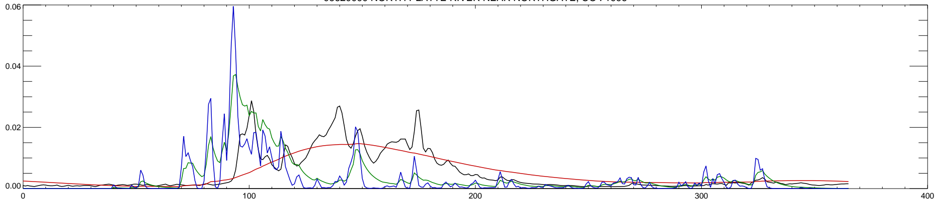
06620000 NORTH PLATTE RIVER NEAR NORTHGATE, CO : 1997
