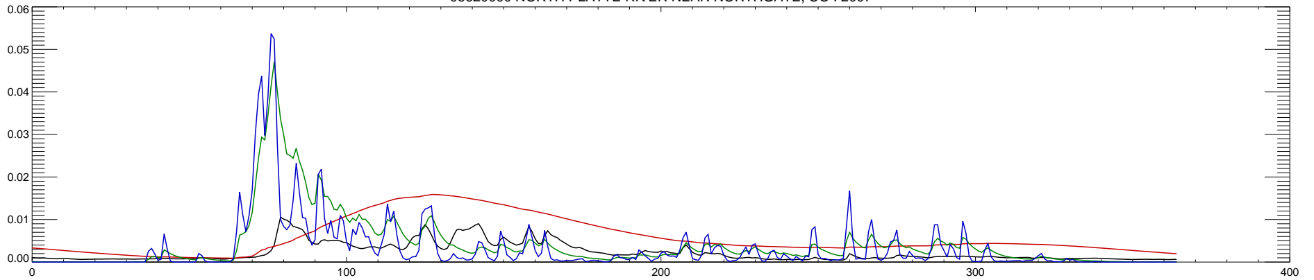
06620000 NORTH PLATTE RIVER NEAR NORTHGATE, CO : 2007
