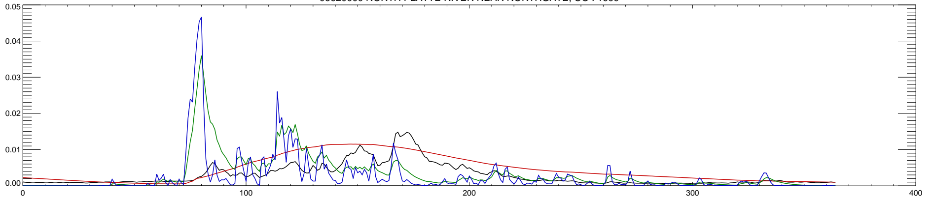
06620000 NORTH PLATTE RIVER NEAR NORTHGATE, CO : 2000
