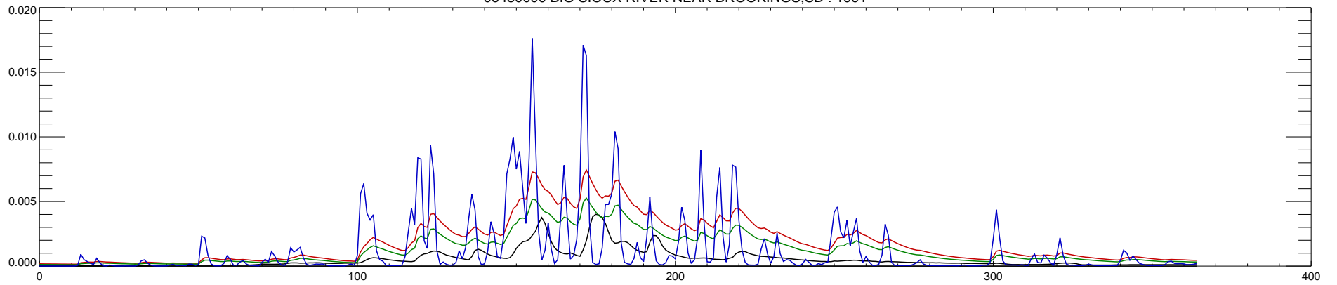
06480000 BIG SIOUX RIVER NEAR BROOKINGS,SD : 1992
