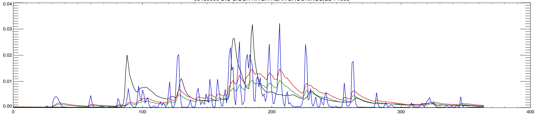
06480000 BIG SIOUX RIVER NEAR BROOKINGS,SD : 1994
