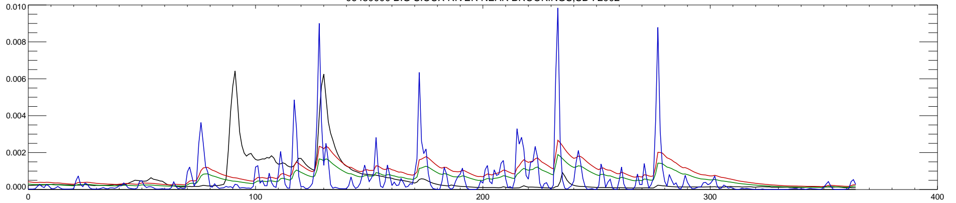
06480000 BIG SIOUX RIVER NEAR BROOKINGS,SD : 2003
