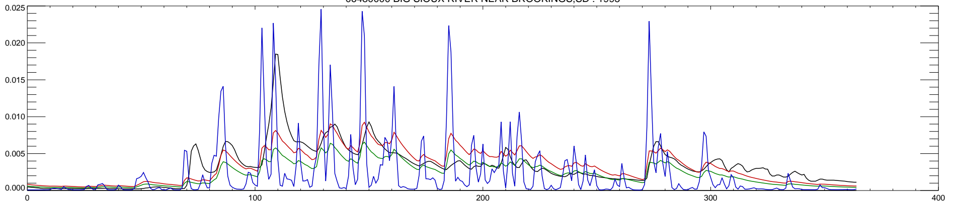
06480000 BIG SIOUX RIVER NEAR BROOKINGS,SD : 1995
