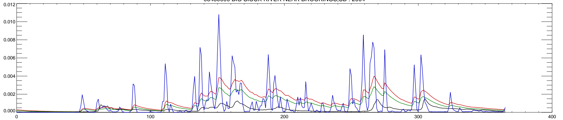
06480000 BIG SIOUX RIVER NEAR BROOKINGS,SD : 2004
