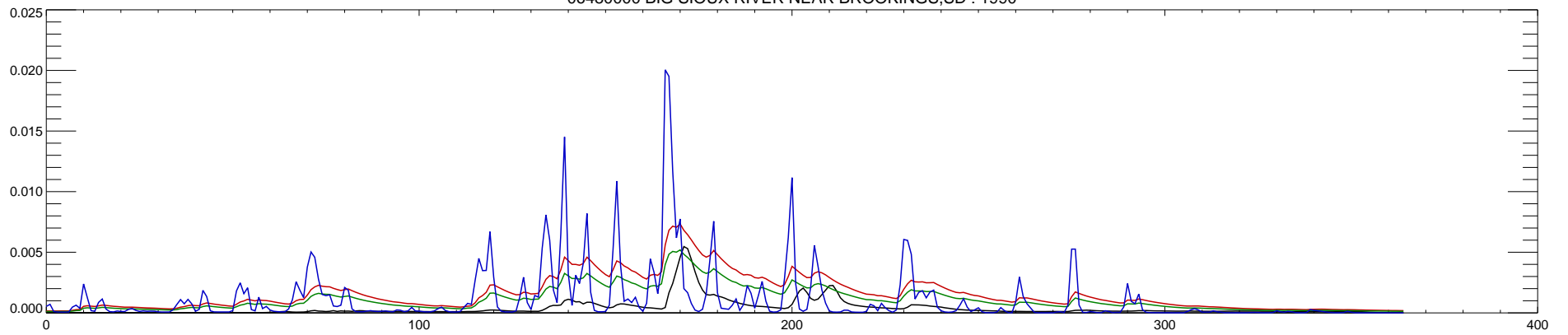
06480000 BIG SIOUX RIVER NEAR BROOKINGS,SD : 1991
