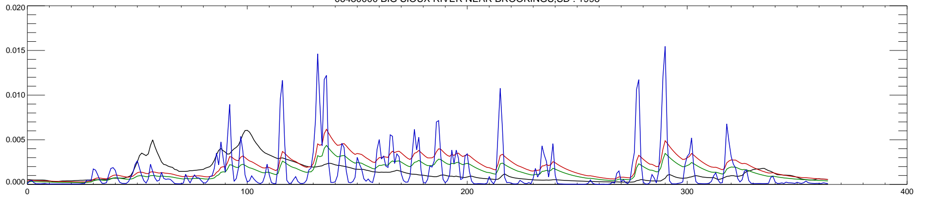
06480000 BIG SIOUX RIVER NEAR BROOKINGS,SD : 1998
