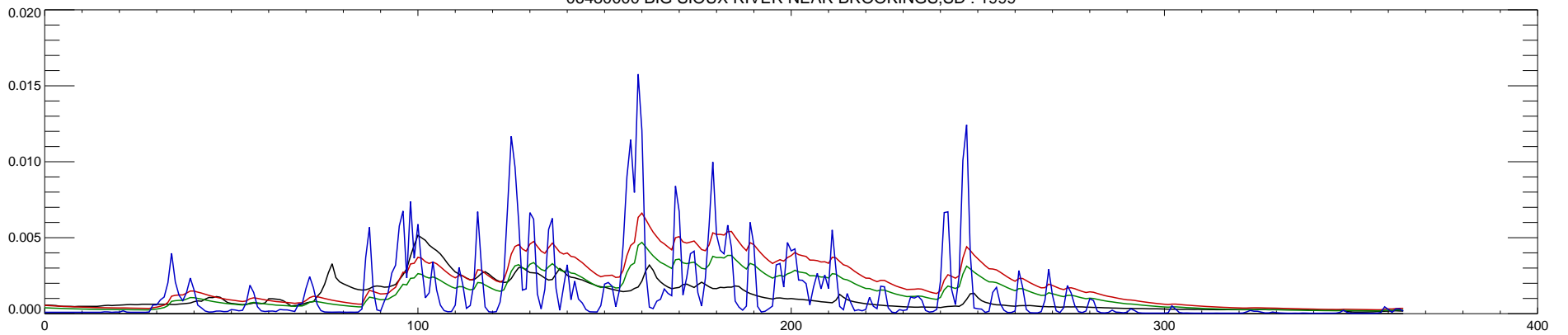
06480000 BIG SIOUX RIVER NEAR BROOKINGS,SD : 2000
