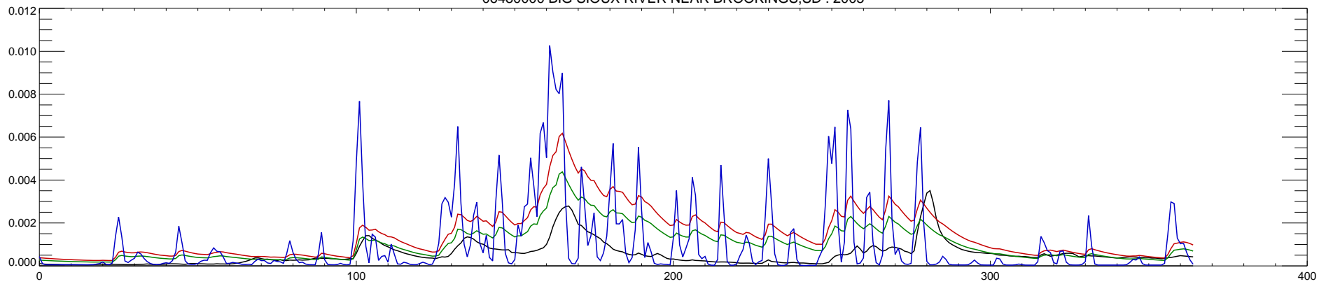
06480000 BIG SIOUX RIVER NEAR BROOKINGS,SD : 2006
