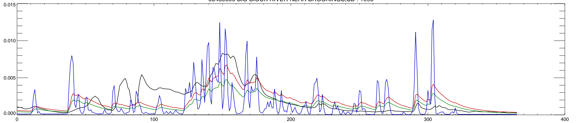
06480000 BIG SIOUX RIVER NEAR BROOKINGS,SD : 1997
