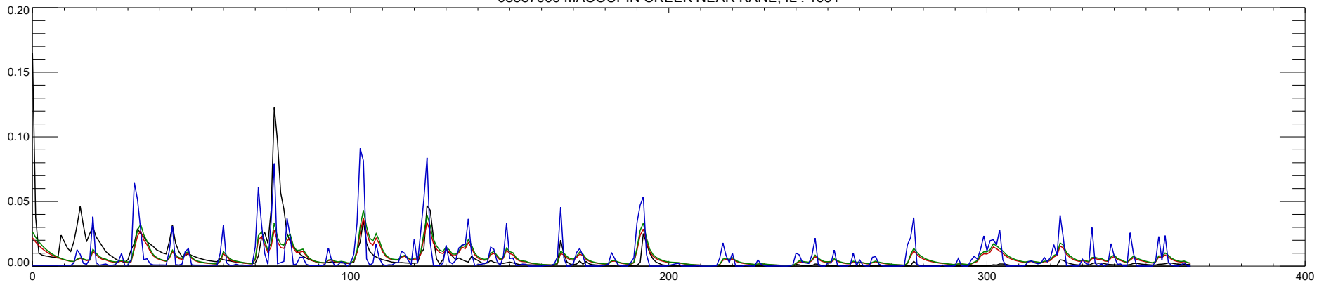
05587000 MACOUPIN CREEK NEAR KANE, IL : 1992
