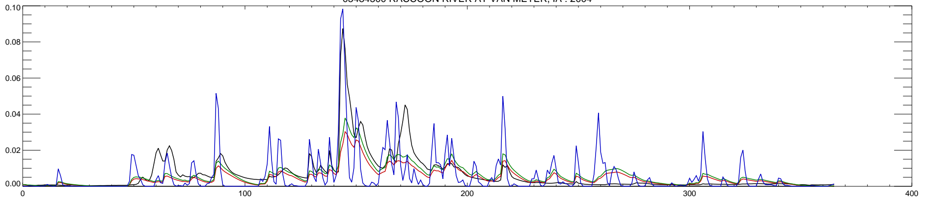
05484500 RACCOON RIVER AT VAN METER, IA : 2004
