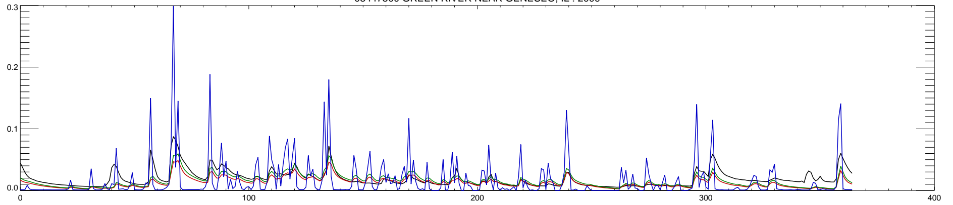
05447500 GREEN RIVER NEAR GENESEO, IL : 2009
