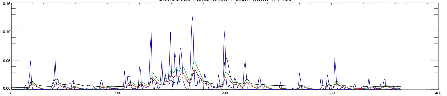
05434500 PECATONICA RIVER AT MARTINTOWN, WI : 1997
