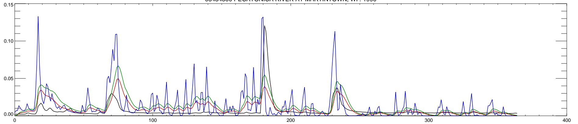
05434500 PECATONICA RIVER AT MARTINTOWN, WI : 1991
