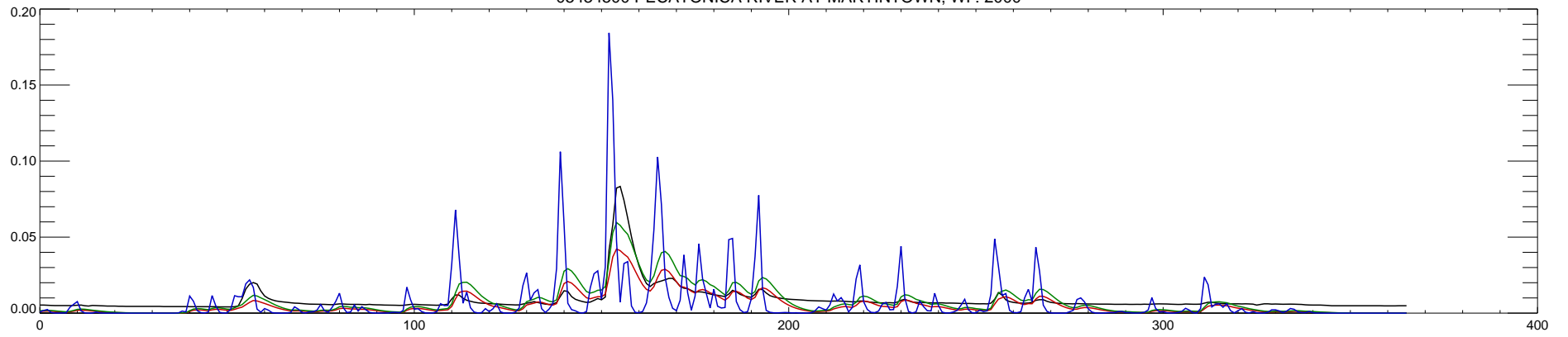
05434500 PECATONICA RIVER AT MARTINTOWN, WI : 2001
