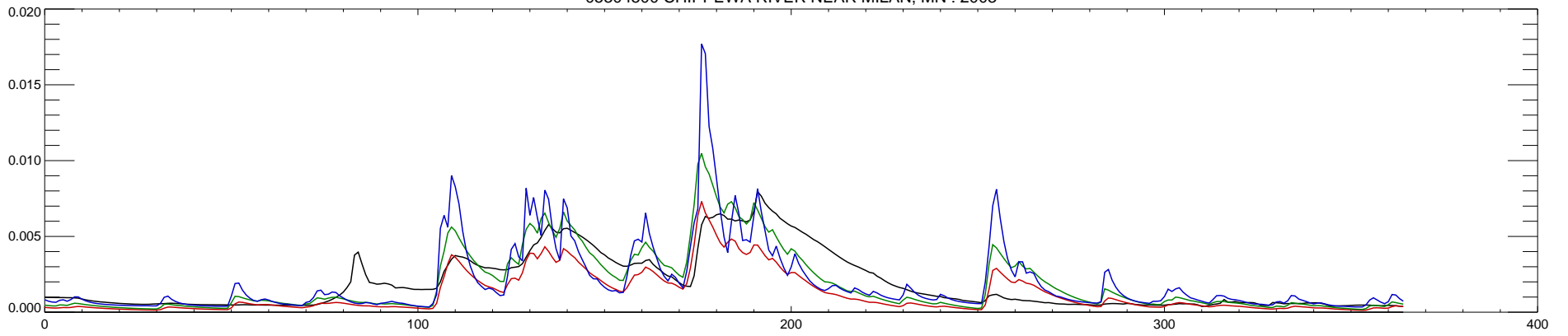
05304500 CHIPPEWA RIVER NEAR MILAN, MN : 2004
