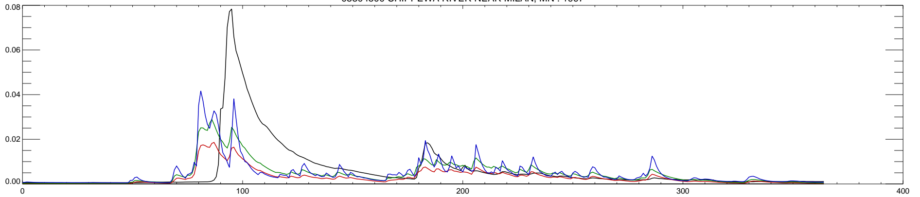
05304500 CHIPPEWA RIVER NEAR MILAN, MN : 1998
