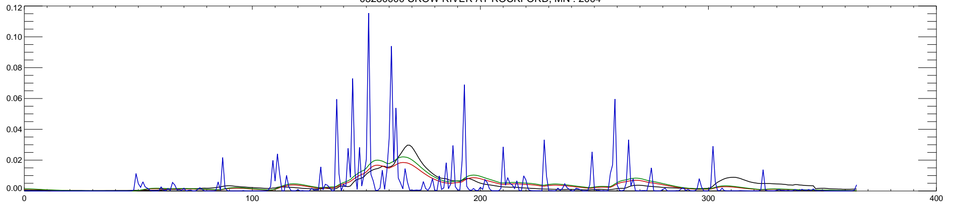
05280000 CROW RIVER AT ROCKFORD, MN : 2004
