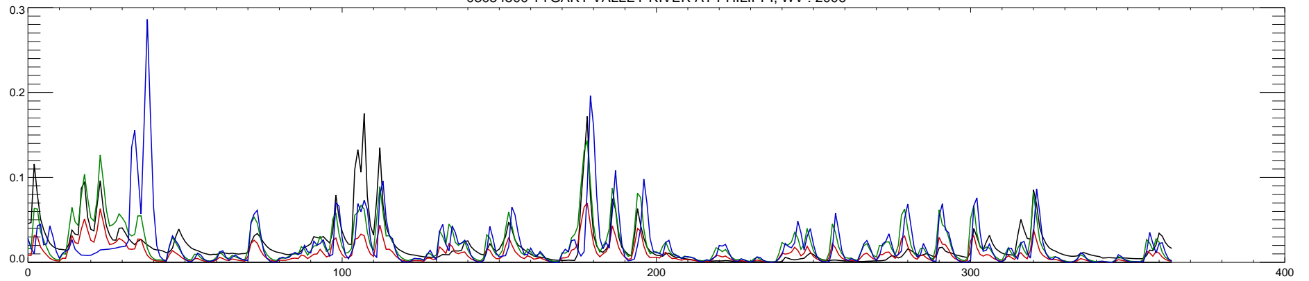
03054500 TYGART VALLEY RIVER AT PHILIPPI, WV : 2007
