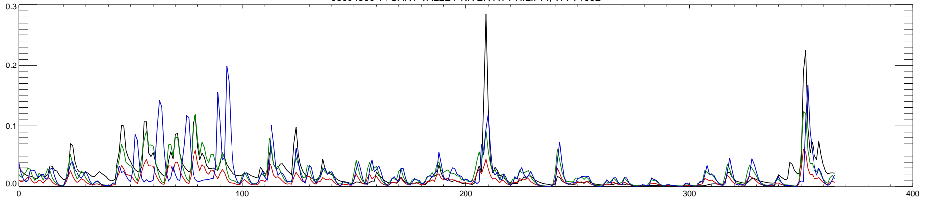
03054500 TYGART VALLEY RIVER AT PHILIPPI, WV : 1992
