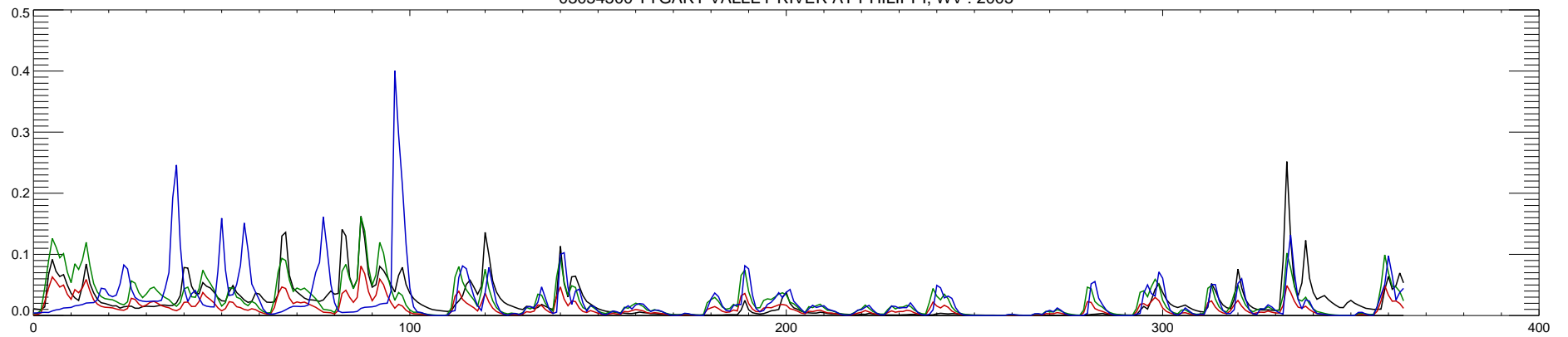
03054500 TYGART VALLEY RIVER AT PHILIPPI, WV : 2006
