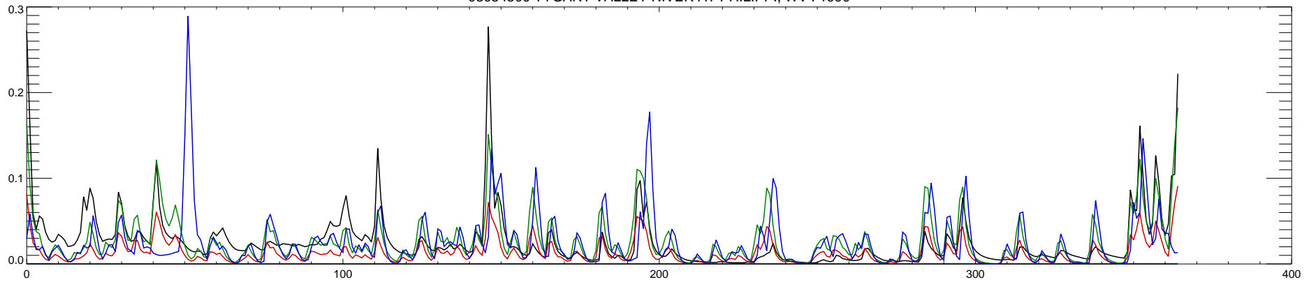
03054500 TYGART VALLEY RIVER AT PHILIPPI, WV : 1991
