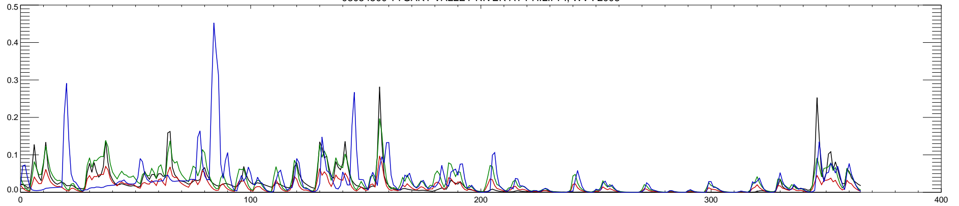
03054500 TYGART VALLEY RIVER AT PHILIPPI, WV : 2009
