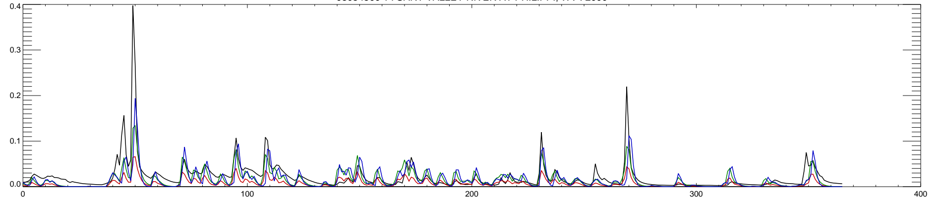
03054500 TYGART VALLEY RIVER AT PHILIPPI, WV : 2001
