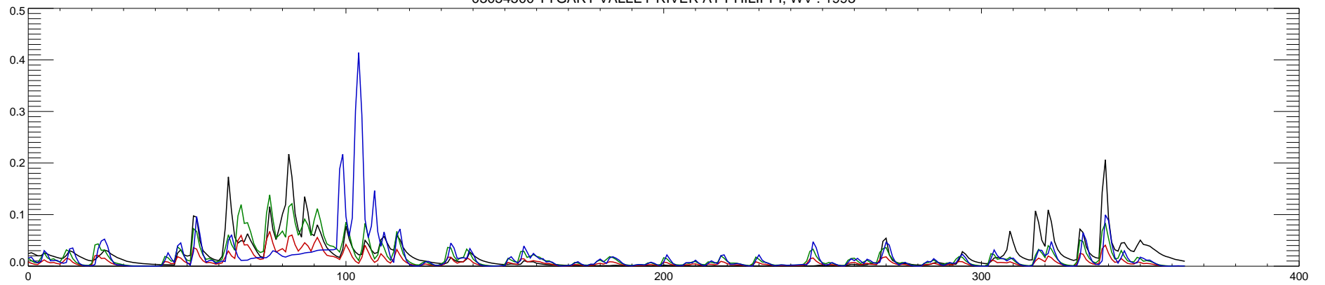
03054500 TYGART VALLEY RIVER AT PHILIPPI, WV : 1994
