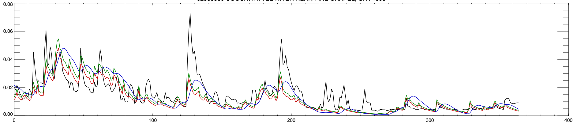
02383500 COOSAWATTEE RIVER NEAR PINE CHAPEL, GA : 2000
