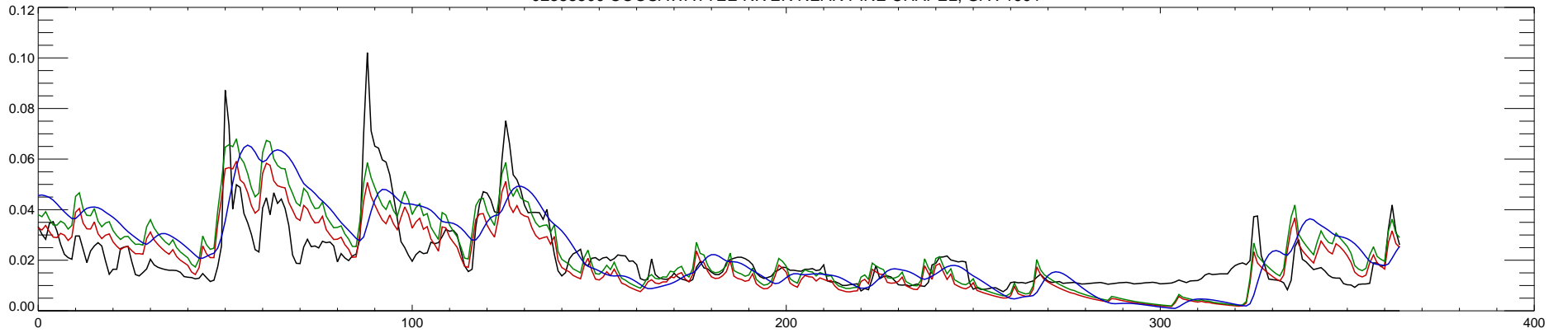
02383500 COOSAWATTEE RIVER NEAR PINE CHAPEL, GA : 1992
